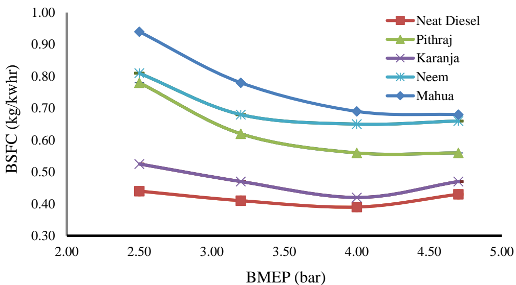
Figure 6. BSFC with different fuels.
