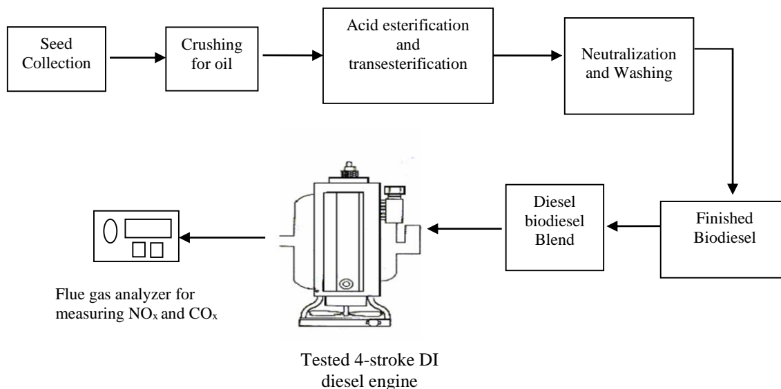
Figure 2. Schematic diagram of the experimental setup.
