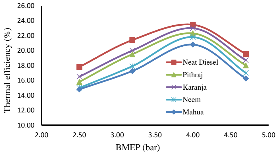
Figure 8. Thermal efficiency with neat diesel and biodiesel blends.
