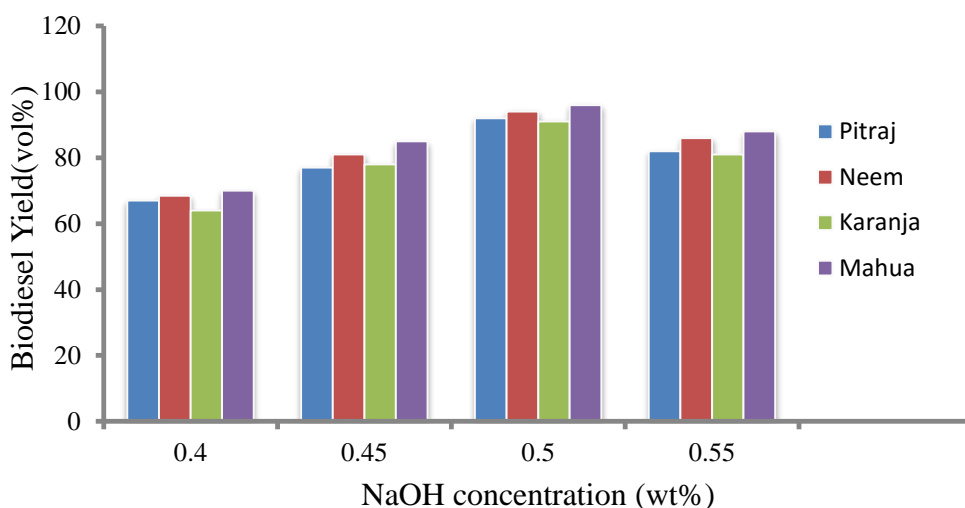
Figure 4. Variation of biodiesel yield with catalyst (NaOH) concentration (temperature=60°C).
