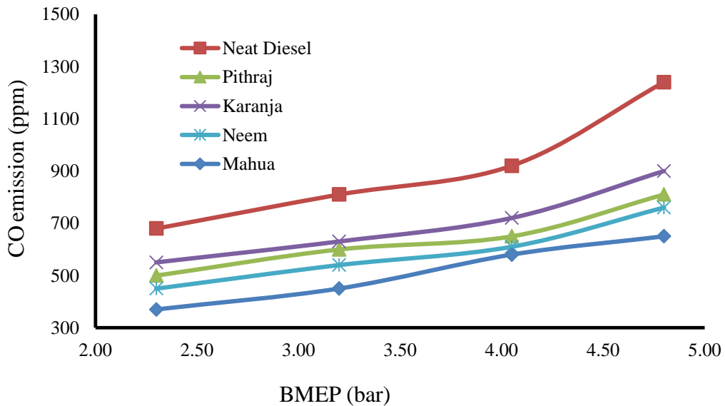
Figure 10. CO emission with neat diesel and different biodiesels.
