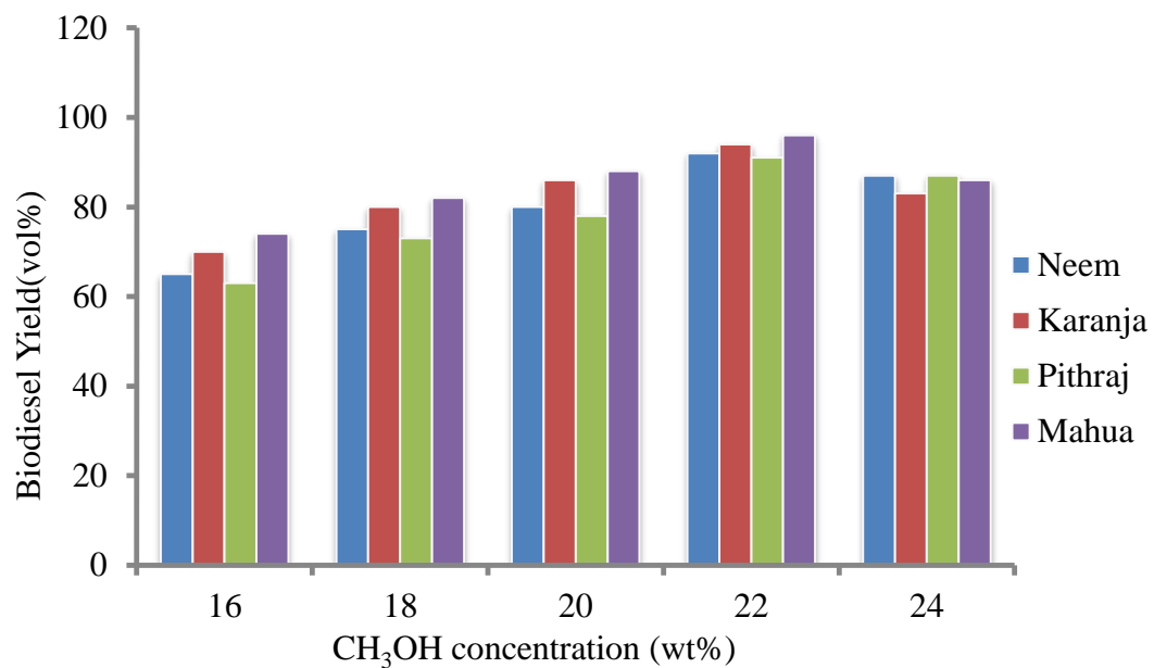
Figure 3. Variation of biodiesel with CH 3 OH % vol.
