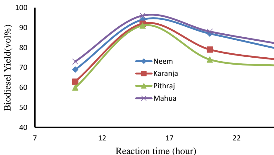
Figure 5. Effect of reaction time on biodiesel production (CH 3 OH = 22%, NaOH = 0.5%).
