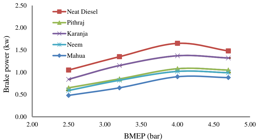
Figure 7. Brake power with neat diesel and various fuels.
