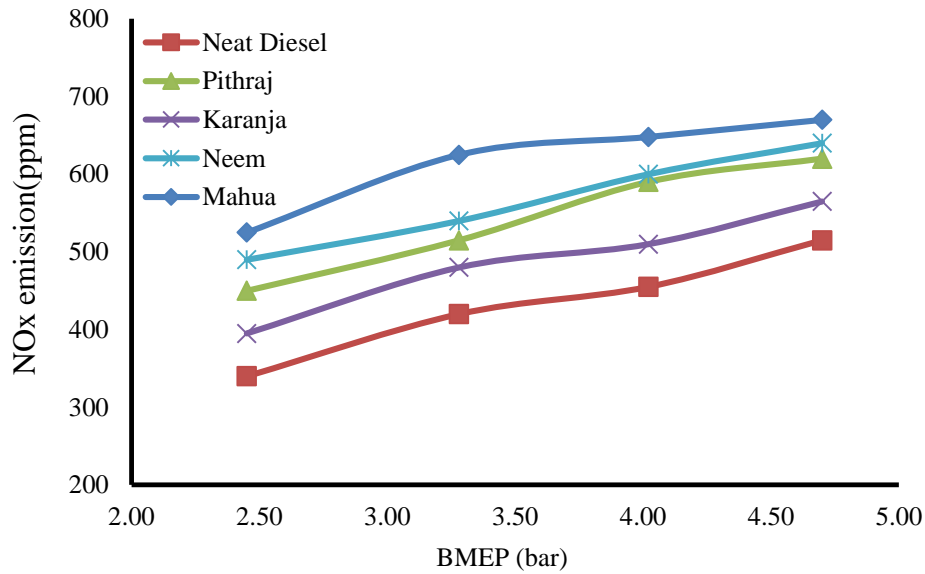
Figure 9. NOx emission with neat diesel and different biodiesels.
