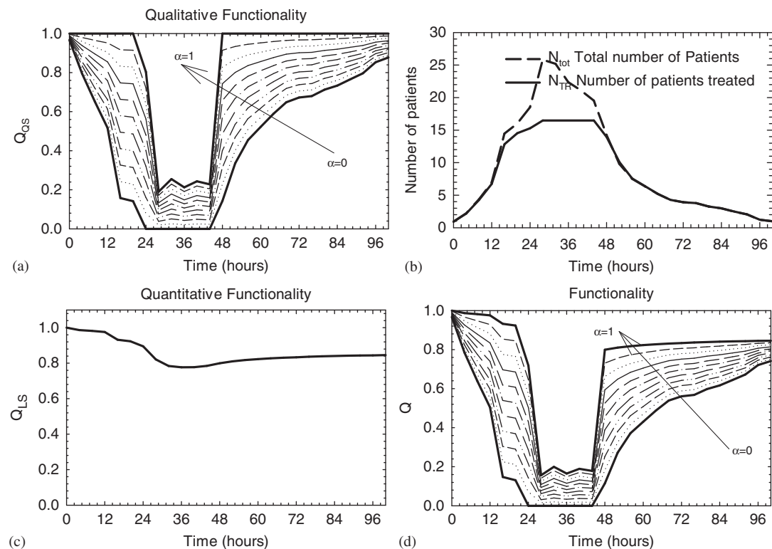
Figure 2. (a) Qualitative functionality for different \alpha factors; (b) Number of patients treated; (c) Quantitative functionality (500 beds, 15 OR, and 1200 classes of efficiency); and (d) Combined functionality Q for different weighting factors.
