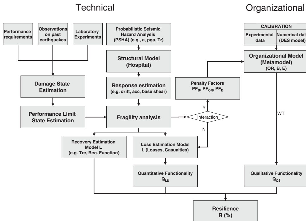
Figure 1. Resilience framework (MCEER approach).
