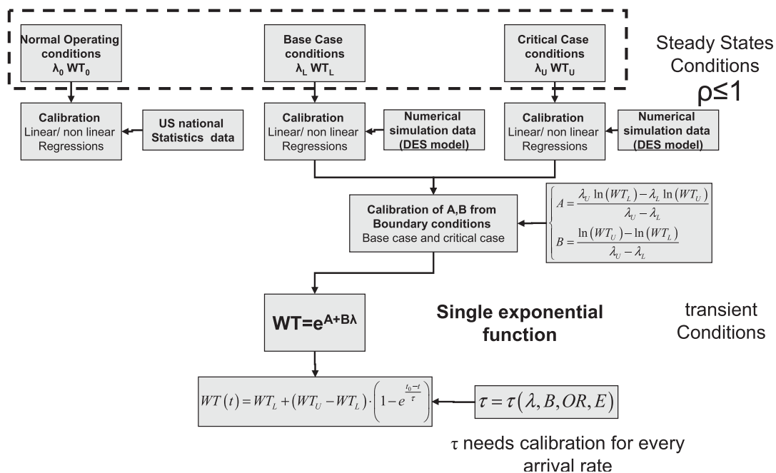
Figure 5. Flowchart of the calibration of the single exponential function.
