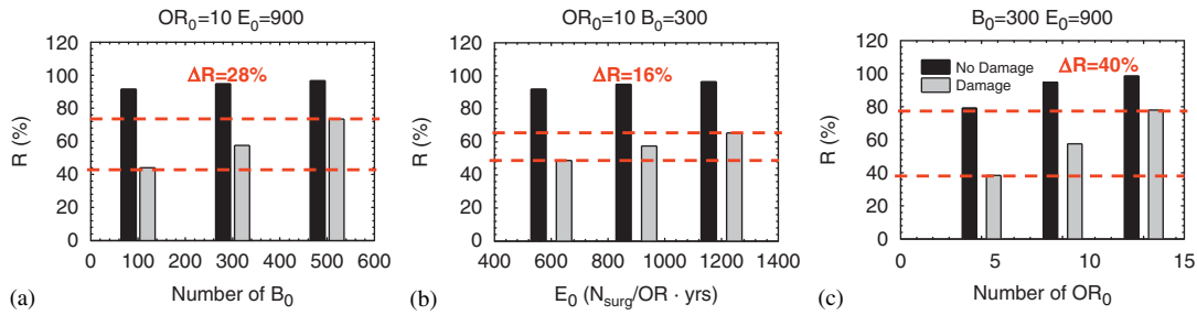
Figure 9. Increments of resilience index vs different internal parameters B , OR and E .
