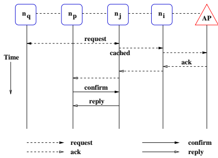
Figure 4. A modified simple search (MSS) algorithm for querying data items in the IMANET.
