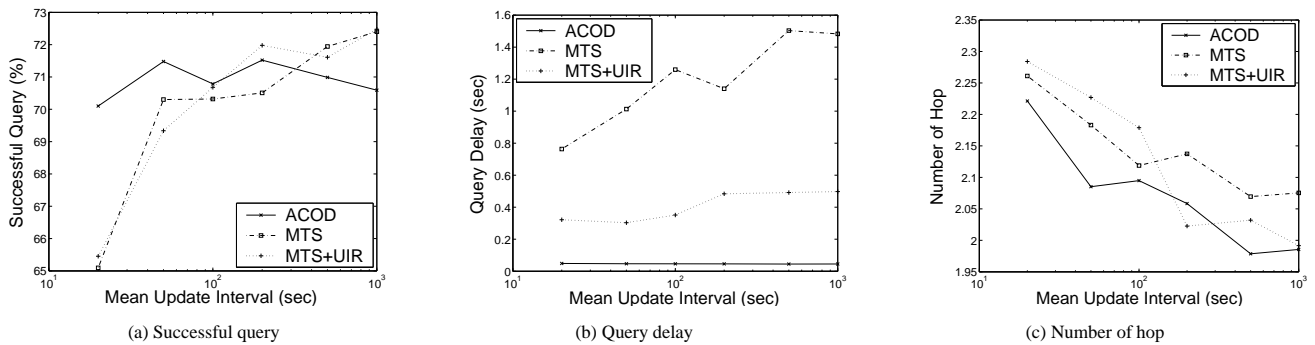
Figure 8. Successful query, query delay, number of hops as a function of mean update interval ( T_{query} = 100 , and C_{size} = 10 ).
