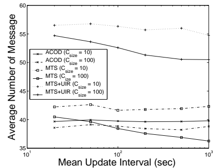
Figure 10. Average number of messages as a function of mean update interval ( T_{query} = 100 , and C_{size} = 10 or 100 ).
