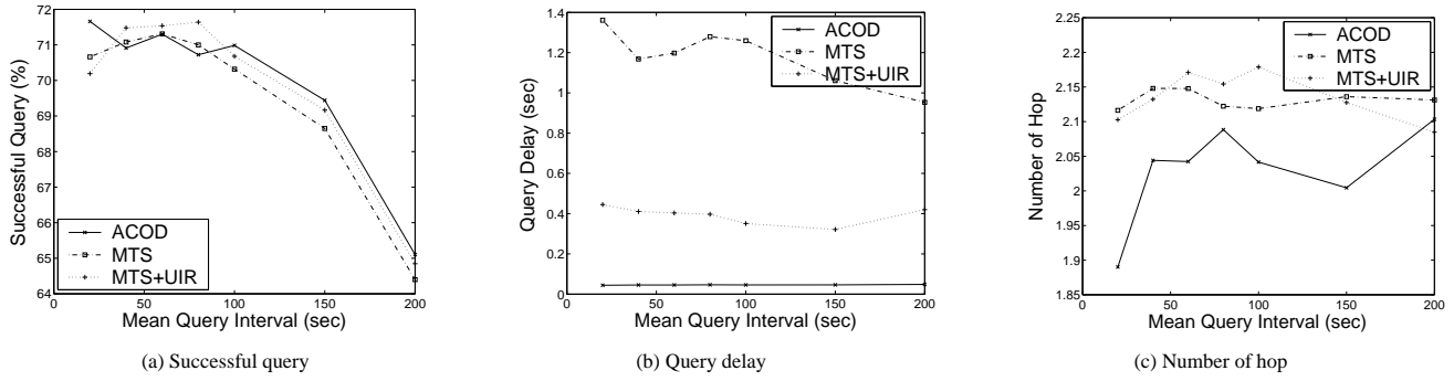
Figure 7. Successful query, query latency, the number of hops as a function of mean query interval ( T_{update} = 100 , and C_{size} = 10 ).
