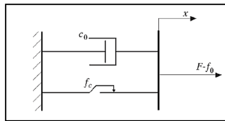
Figure 3: Schematic of Bingham model
