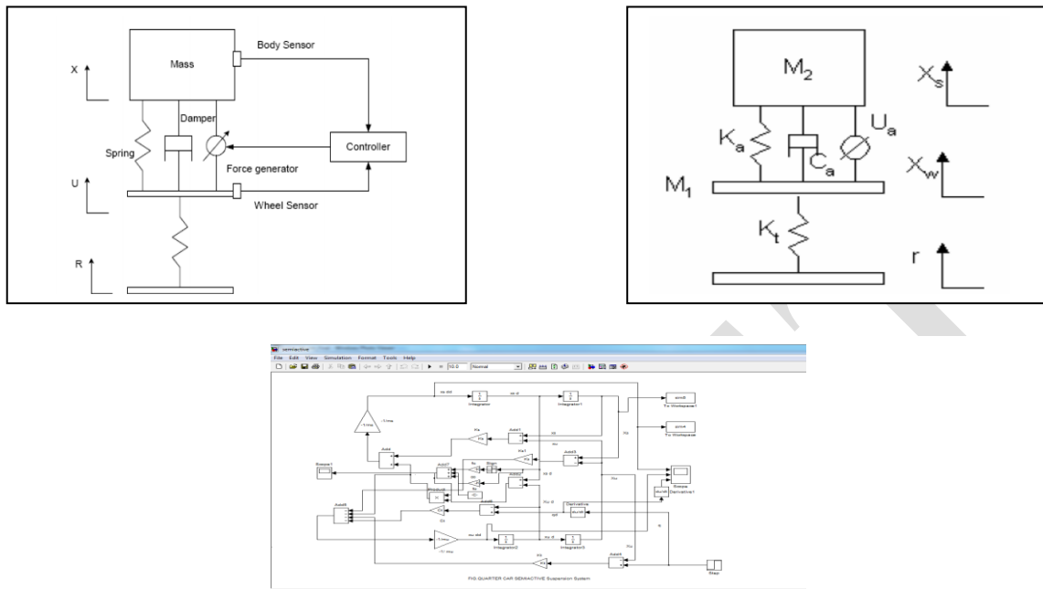
Figure 5 : MATLAB/Simulink Model of Semiactive Suspension System based on Bingham Model
