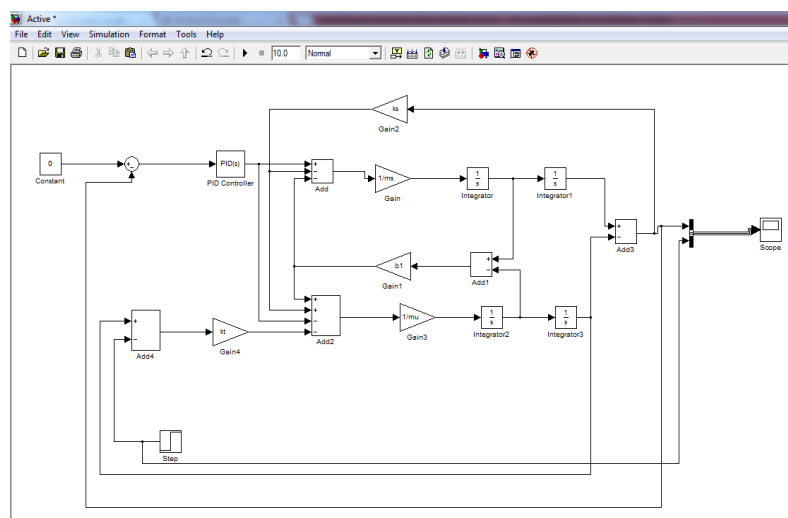
Figure 6 : MATLAB/Simulink Model of active Suspension System based on Bingham Model
