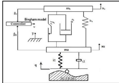
Figure 4: Quarter car vehicle with MR damper
