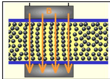
Figure1: Schematic of a magneto rheological fluid
