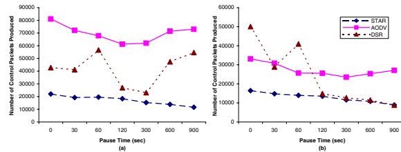
Fig. 14. Control Overhead in Scenario 5 for (a)60 (b)20 Data Flows
