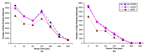
Fig. 7. Data Delivery in Scenario 3 for (a)60 (b)20 Data Flows
