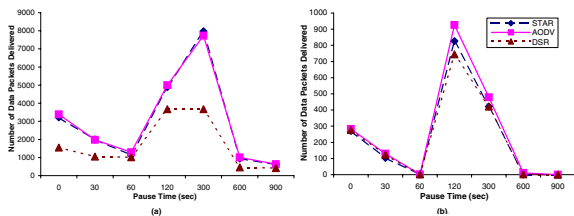
Fig. 4. Data Delivery in Scenario 2 for (a)60 (b)20 Data Flows
