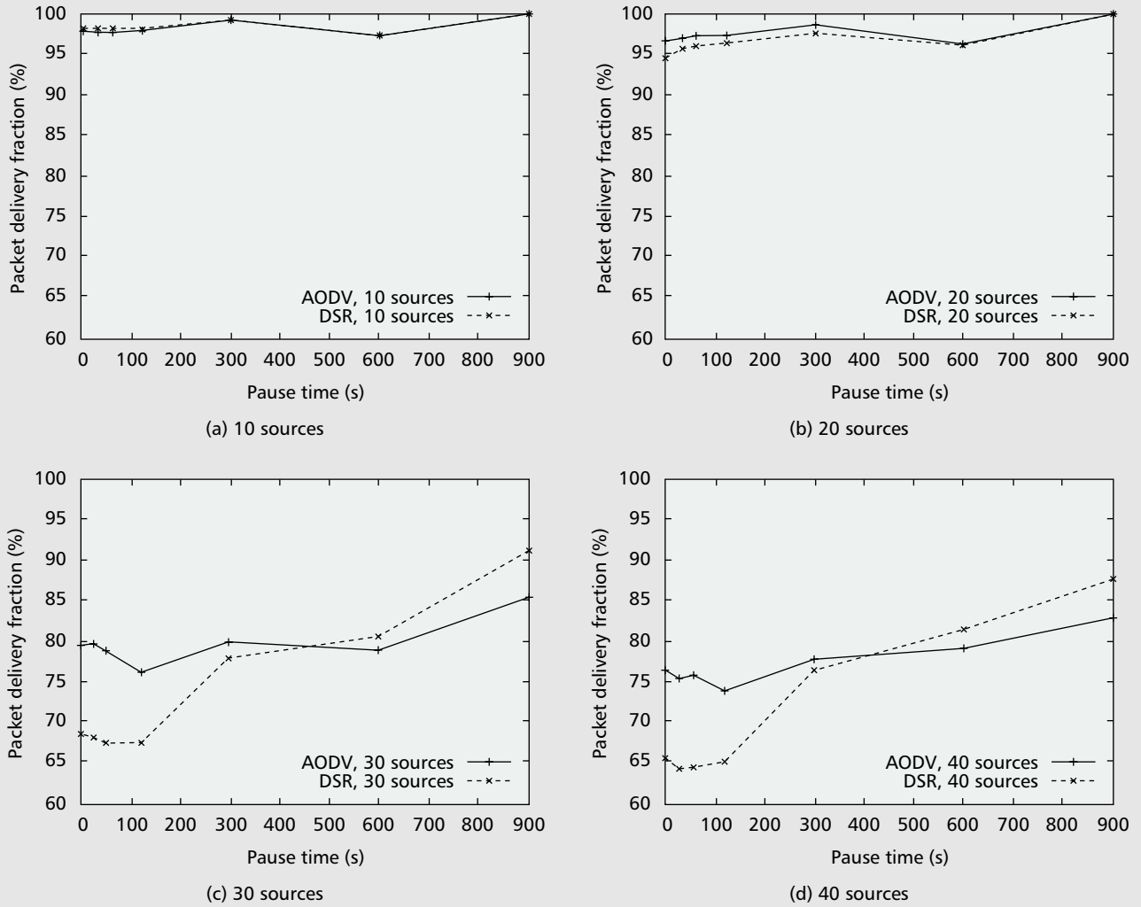
■ Figure 1. Packet delivery fractions for the 50-node model with various numbers of sources.
