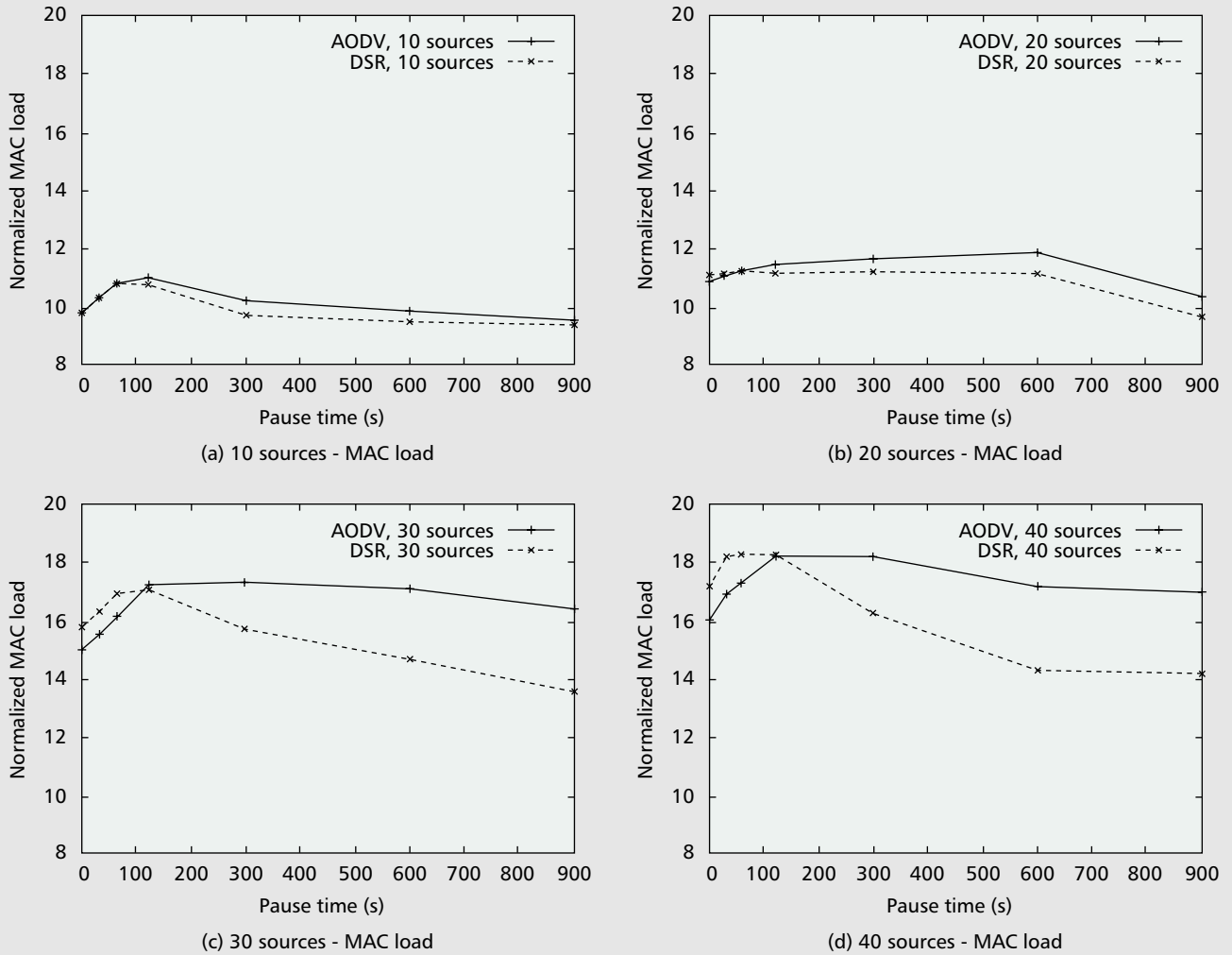
■ Figure 4. Normalized MAC loads for the 50-node model with various numbers of sources.
