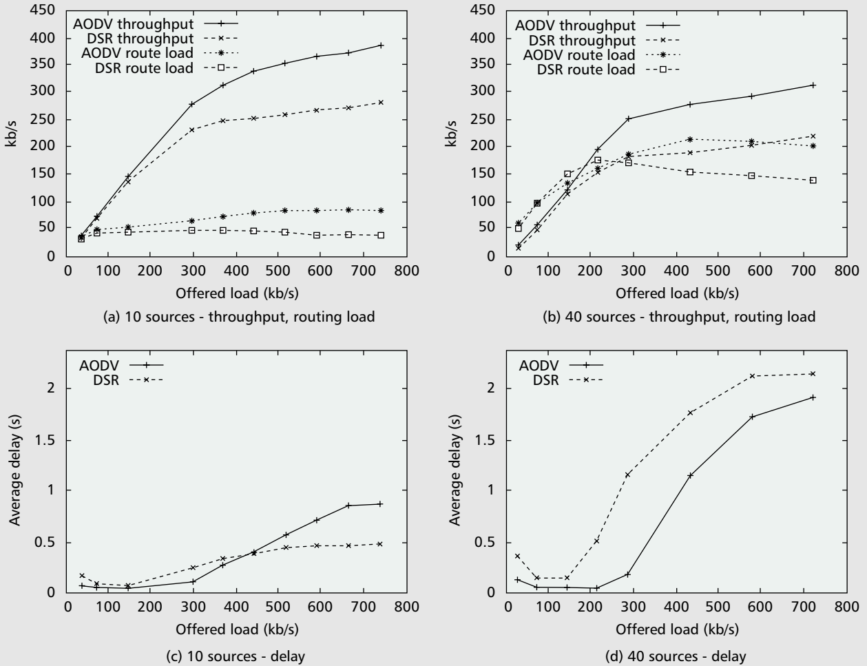
■ Figure 7. Performance with increasing offered load for 100 nodes with 10 and 40 sources.
