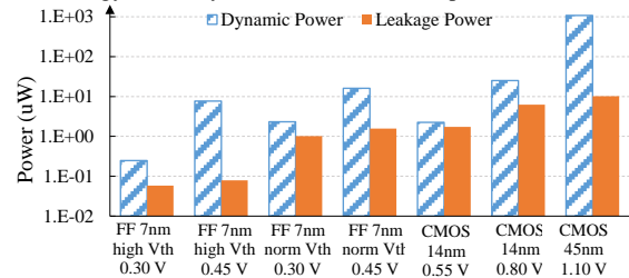
Figure 11. Dynamic and leakage power consumptions of the c3540 benchmark for different standard cell libraries.
