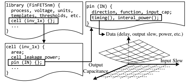
Figure 2. Hierarchy of Liberty format library.
