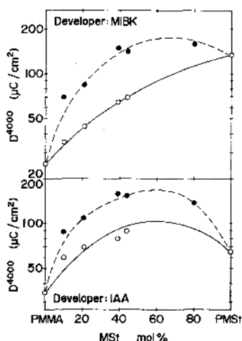
Figure 11. Effect of composition on the sensitivity: ○, copolymer; ●, blend.
