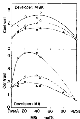
Figure 10. Effect of composition on the contrast: ○, \gamma of copolymer; △, \gamma' of copolymer; ▲, \gamma' of blend.
