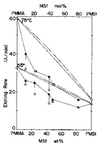
Figure 13. Effect of composition on the dry etching rate: ○, △, copolymer; ●, ▲, blend. Broken and chain lines indicate weight- and mol-percent addivities, respectively.
