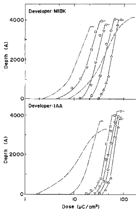
Figure 8. Effect of copolymerization ratio on the characteristics: — —, PMMA; □, C-10; ▽, C-21; ◇, C-39; △, C-44; ·····, P-35.
