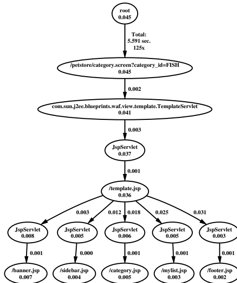
Figure 14: PetStore results, normal configuration (nesting algorithm)
