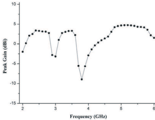
Figure 6. Gains of the antenna versus different frequencies.
