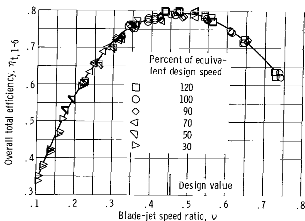
(b) Total efficiency.
