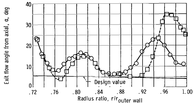
(b) Exit flow angle.
