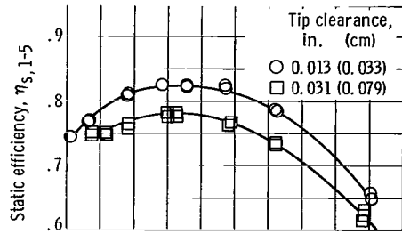
(a) Static efficiency.
