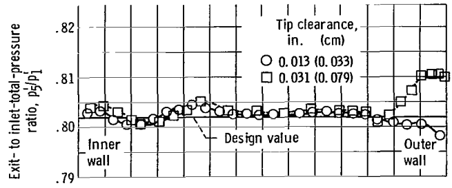
(a) Exit total pressure.
