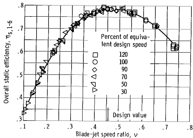
(a) Static efficiency.
