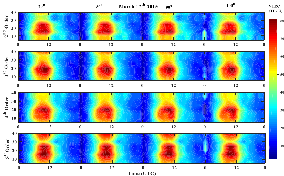
FIGURE 3. EIA peak recognition at 70°E, 80°E, 90°E, 100°E longitudes on geomagnetic disturbed day 17-03-2015.
