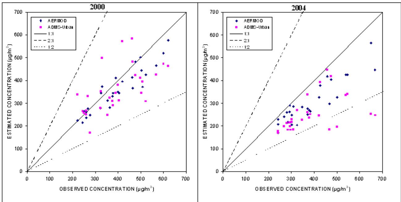
Fig. 5. Scatter plots of estimated vs. observed monthly average TSPM concentrations (Left: Year 2000, Right: Year 2004).
