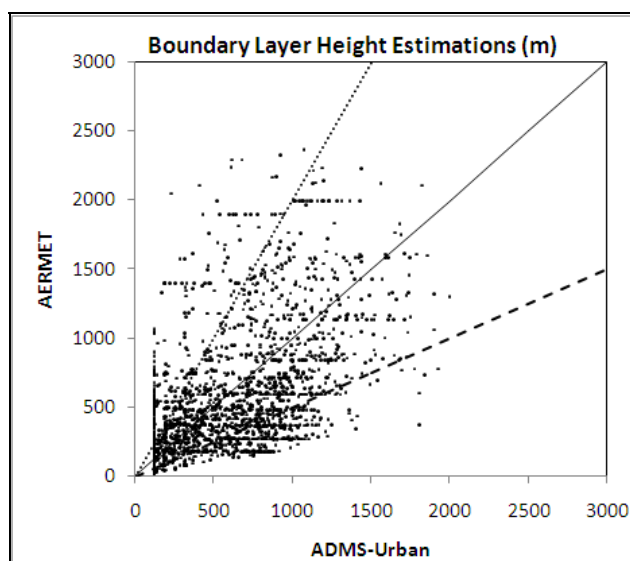
Fig. 9. Boundary layer height estimations (meters) by AERMET and meteorological processor of ADMS-Urban for years 2000 and 2004.
