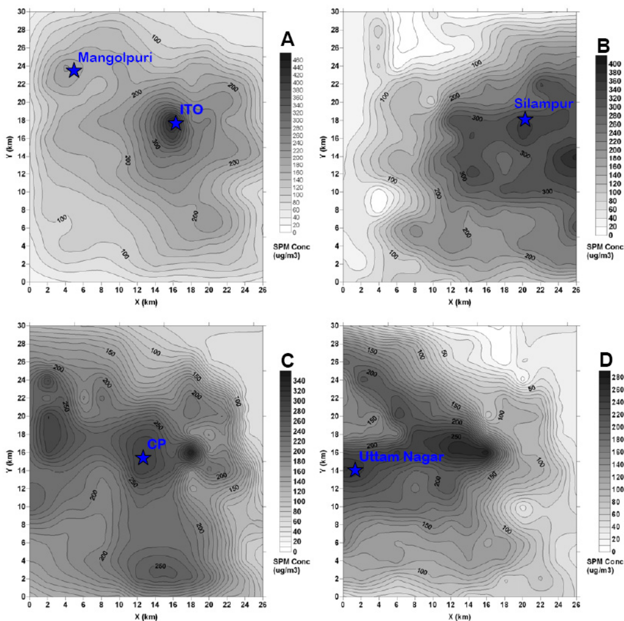
Fig. 8. Concentration isopleths for TSPM as estimated by (A) AERMOD, year 2000 (B) ADMS-Urban, year 2000; (C) AERMOD, year 2004; (D) ADMS-Urban, year 2004.
