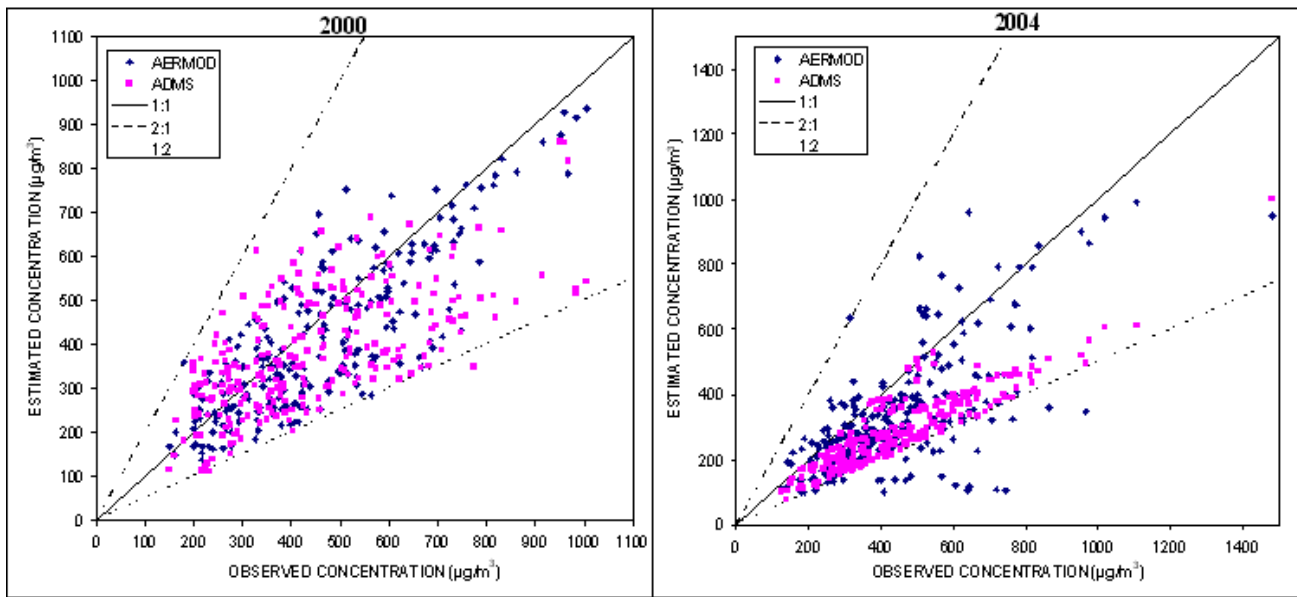
Fig. 4. Scatter plots of estimated vs. observed daily average TSPM concentrations (Left: Year 2000, Right: Year 2004).
