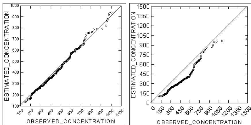
Fig. 6. Q–Q plots of estimated (by AERMOD) and observed daily average TSPM concentrations for years 2000 (left) and 2004 (right). All concentration units are in \mu\text{g}/\text{m}^3 .
