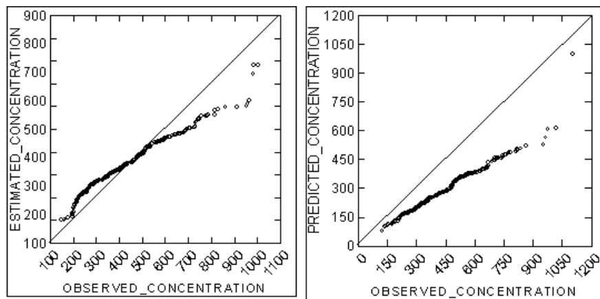
Fig. 7. Q–Q plots of estimated (by ADMS-Urban) and observed daily average TSPM concentrations for years 2000 (left) and 2004 (right). All concentration units are in \mu\text{g}/\text{m}^3 .
