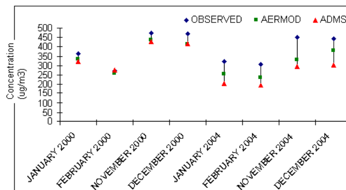
Fig. 3. Comparison of monthly average observed and estimated values of TSPM.
