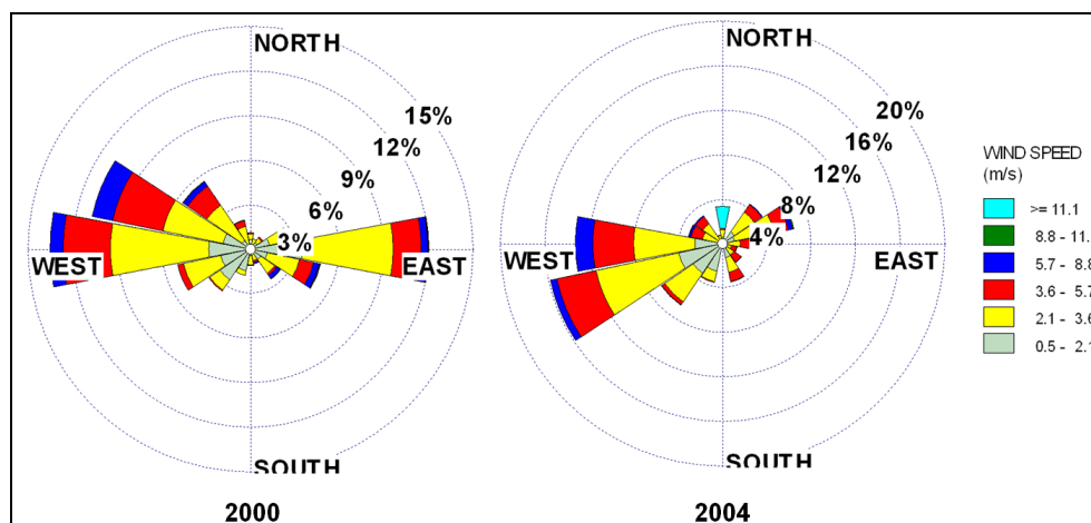
Fig. 2. Wind Roses for winter months (Jan, Feb, Nov, Dec) of year 2000 (left) and year 2004(right).
