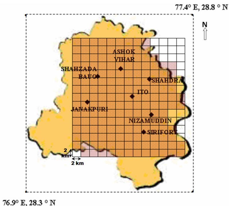
Fig. 1. Grid network (2 km 2 square grid of uniform size throughout the study area) depicting the ambient air quality monitoring stations over the study area of Delhi.
