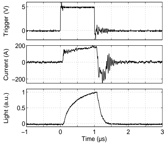
Fig. 2 Circuit response to trigger input for a 1 \mu\text{s} , 200 A pulse with relative LED response in arbitrary units (a.u.)
