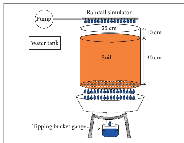
Figure 2. Schematic of the micro-lysimeter.
