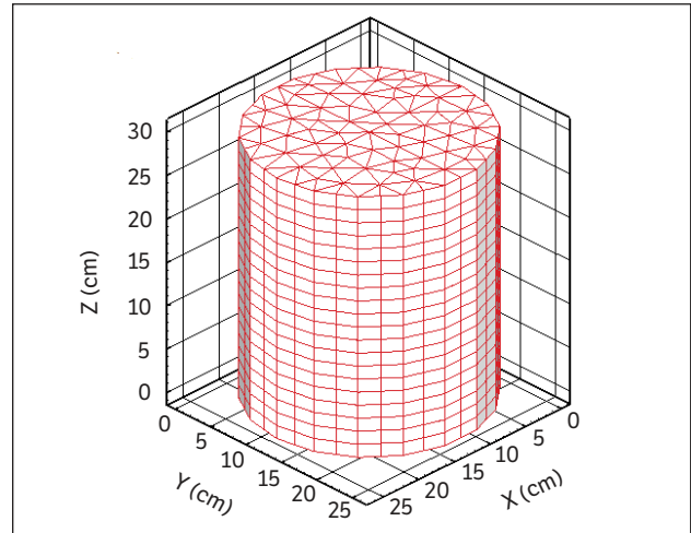
Figure 3. Numerical model mesh.
