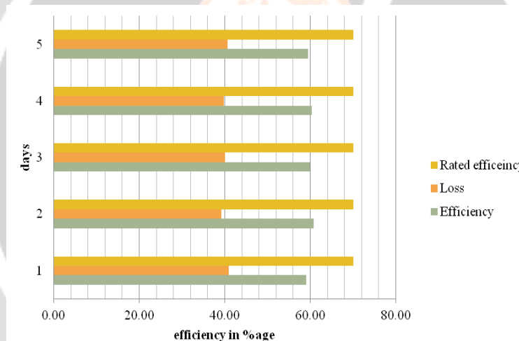
Chart.4 efficiency of boiler
