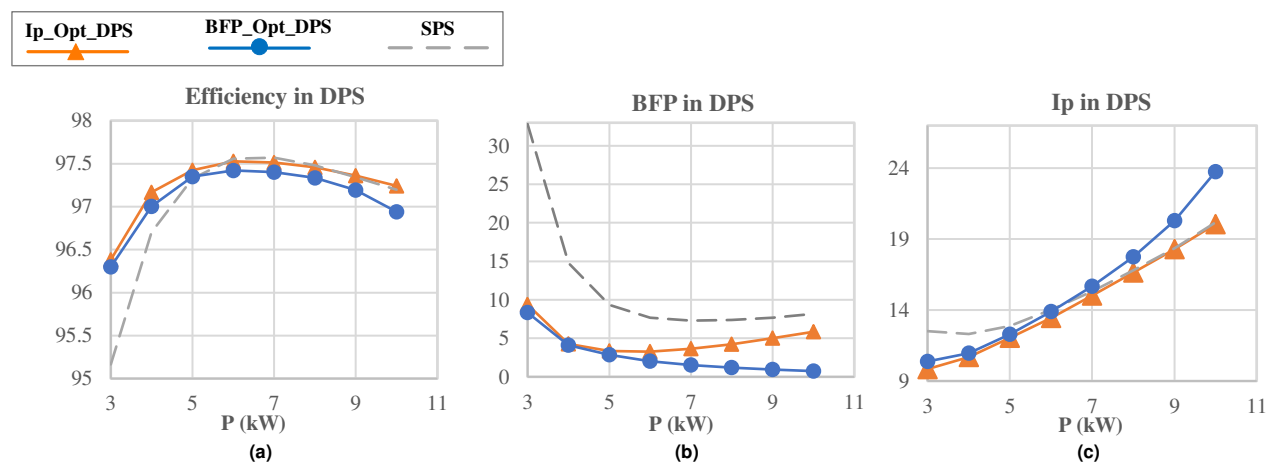
FIGURE 21. The simulation results using the proposed optimization in the “DPS” modulation. (a) the efficiency, (b) the BFP, (c) the peak current. The DPS variants accompanied by BFP and I_p optimization are called BFP_Opt_DPS and Ip_Opt_DPS, respectively.
