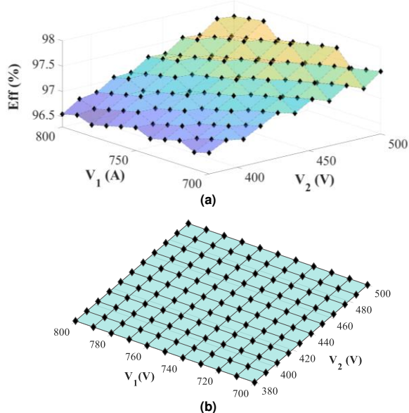
FIGURE 16. The efficiency in the SPS modulation at the nominal power, 10kW (a) the efficiency curve of the SPS-controlled DAB, (b) the selected test points from the voltage range.
