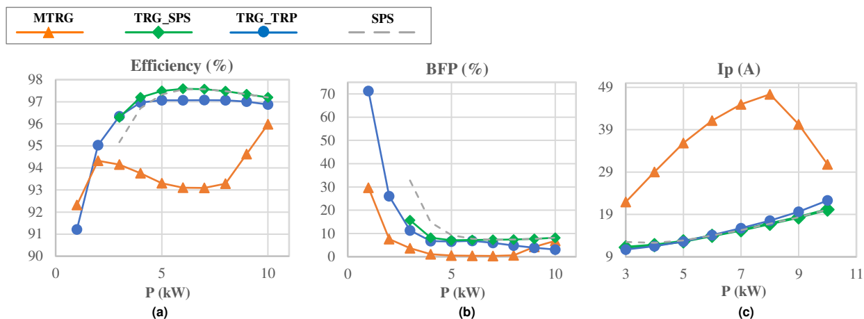
FIGURE 19. The simulation results of the DAB converter, controlled by MTRG and the combinational method, including TRG_SPS and TRG_TRP (a) the efficiency, (b) the BFP, (c) the peak current.
