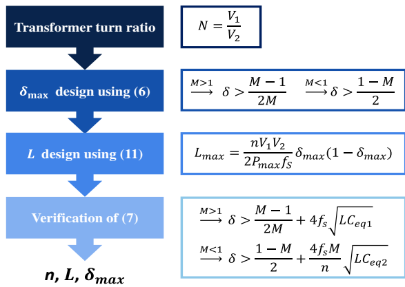
FIGURE 7. A simple design procedure for a DAB converter.
