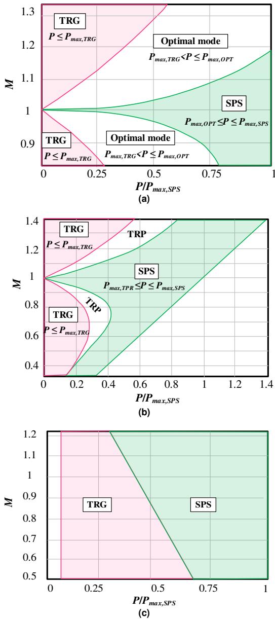
FIGURE 12. The control maps in the literature, (a) the DAB in [37]: P = 2\text{ kW} , 240 < V_1 < 450 , 11 < V_2 < 16 , N = 19 , (b) the DAB in [38]: P = 1.5\text{ kW} , 240 < V_1 < 440 , 6 < V_2 < 16 , N = 24 , (c) the DAB in [34]: P = 1.2\text{ kW} , 28 < V_1 < 45 , 300 < V_2 < 400 , 1/N = 12 .
