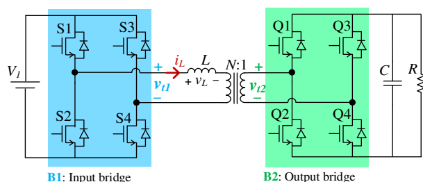
FIGURE 1. The main structure of a single-phase DAB converter.
