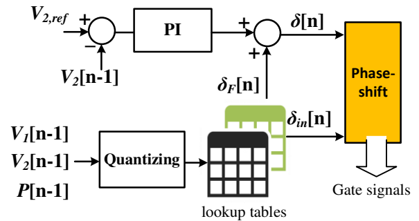
FIGURE 15. The main controller in the designed DAB converter employing optimal values of inner and outer shifts.
