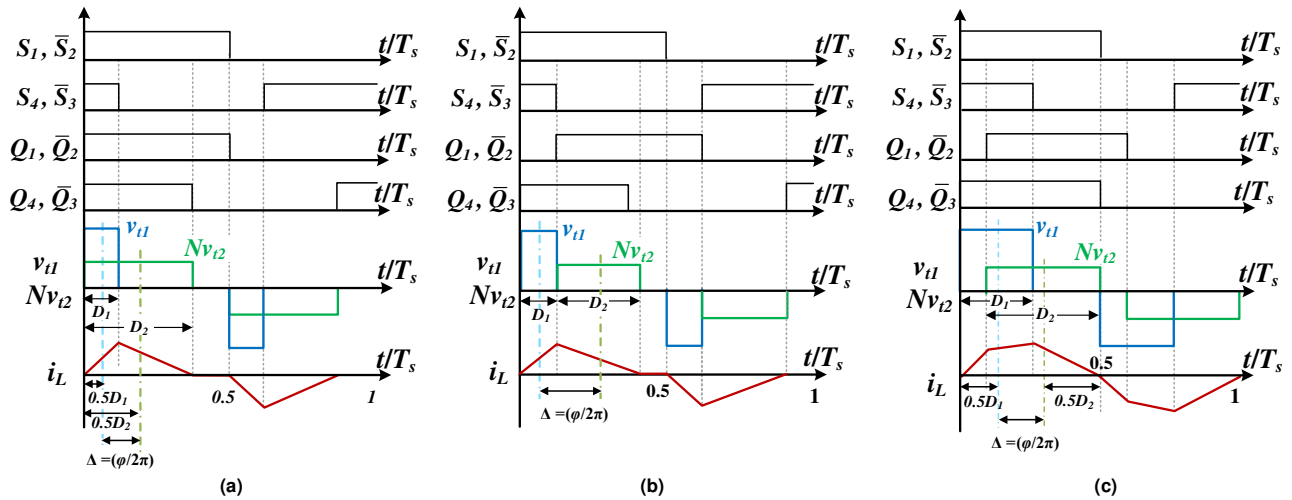
FIGURE 10. Typical waveforms of v_{t1} , Nv_{t2} , i_L for V_1 > Nv_2 and P_{TRG} > 0 in (a) TRG, (2) MTRG, (3) TRP.
