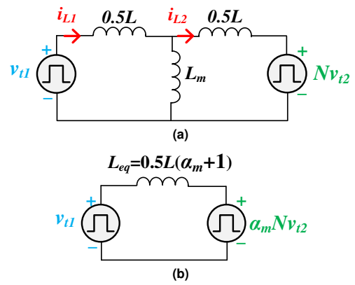
FIGURE 6. The transformer of a DAB, considering the magnetizing inductance, (a) T-model of the transformer, along with the pulsating voltage sources, (b) the simplified model.
