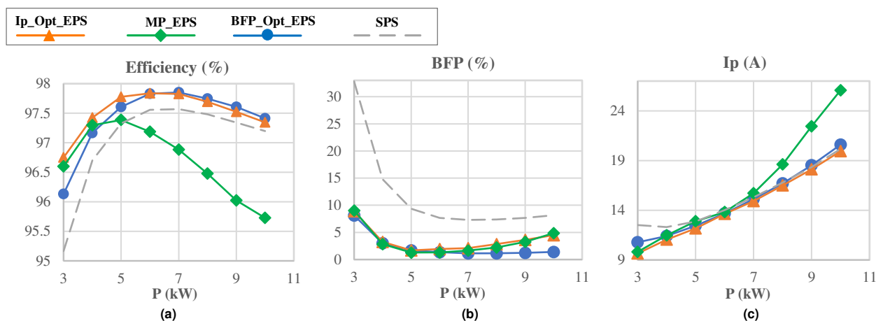
FIGURE 20. The simulation results using the proposed optimization in the “EPS” modulation. (a) the efficiency, (b) the BFP, (c) the peak current. The EPS variants accompanied by BFP and I_p optimization are called BFP_Opt_EPS and Ip_Opt_EPS, respectively. The MP_EPS modulation represents the maximum power EPS method in [16].
