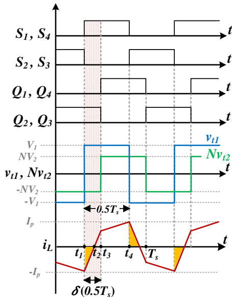
FIGURE 3. Typical waveforms of the gate signals, v_{t1} , Nv_{t2} and i_L in SPS.
