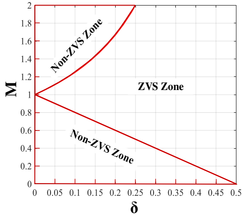
FIGURE 5. The ZVS and non-ZVS zones associated with M and \delta , M = NV_2/N_1 .
