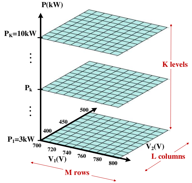
FIGURE 14. Working span division into K levels and M \times L number of segments on each level.
