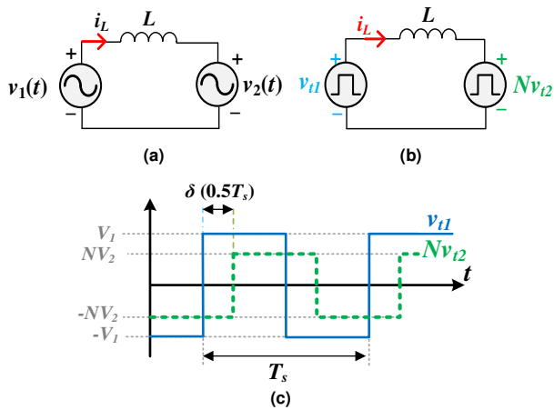
FIGURE 2. Power transmission between two voltage sources. (a) The traditional sinusoidal system, (b) the simplified equivalent circuit of ta DAB converter, (c) the 50% bipolar pulsating voltages.
