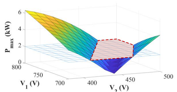
FIGURE 17. The maximum TRG power in the voltage range. For P = 2kW , 40% of the voltage range is not covered by TRG; this area is surrounded with the dashed lines as an example.
