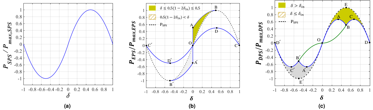
FIGURE 9. The power characterization of the EPS control. (a) the SPS modulation, (b) the EPS modulation, (c) the DPS modulation.
