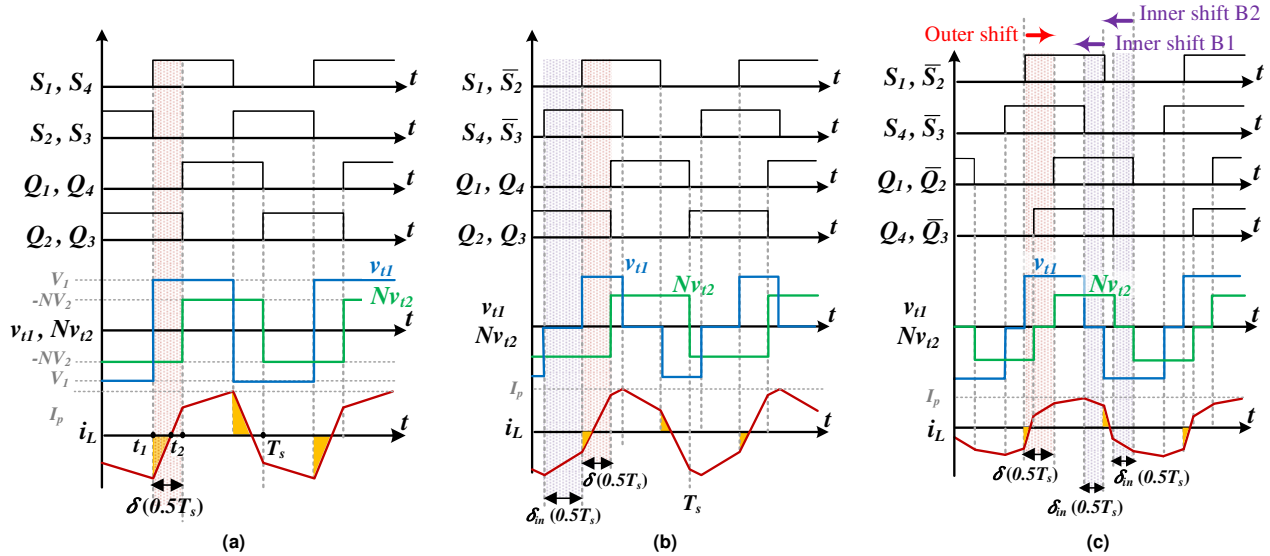
FIGURE 8. Typical waveforms of v_{t1} , Nv_{t2} , i_L and the gate signals ( 0 \leq \delta_{in} \leq 1 ) (a) the SPS modulation, (b) the EPS modulation, (c) the DPS modulation.
