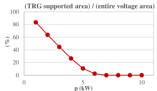
FIGURE 18. The relative value of the TRG manageable area to the entire voltage range in the designed DAB converter.
