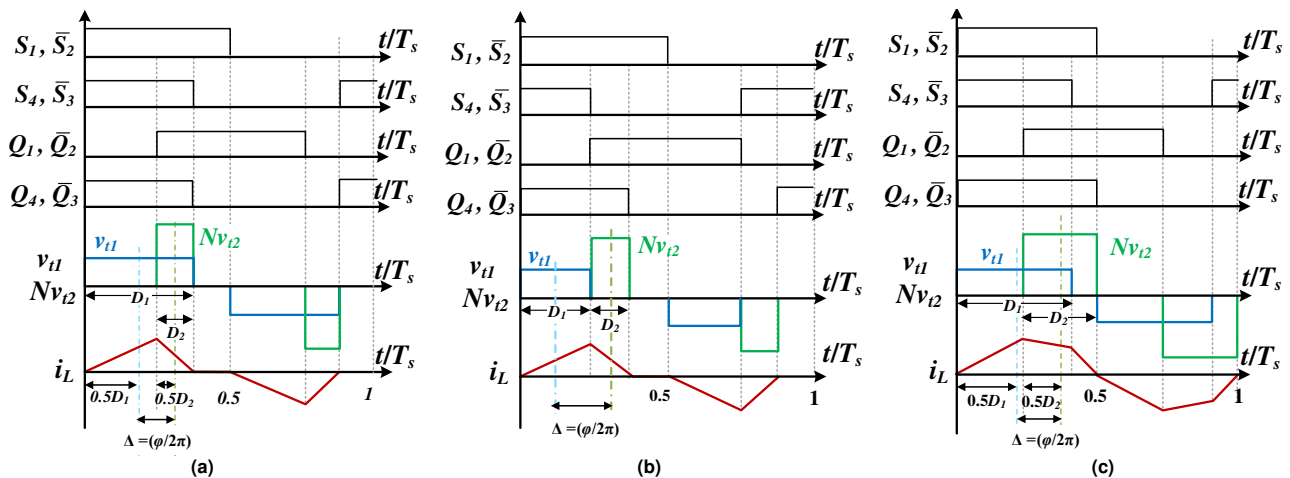
FIGURE 11. Typical waveforms of v_{t1} , Nv_{t2} , i_L for V_1 < Nv_2 and P_{TRG} > 0 in (a) TRG, (2) MTRG, (3) TRP.
