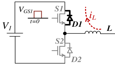
FIGURE 4. The visual clarification of ZVS at S1's turn-on moment.
