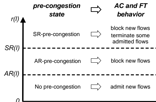
Fig. 1. The admissible and the supportable rate ( AR(l), SR(l) ) define three pre-congestion states concerning the PCN traffic rate r(l) on a link.
