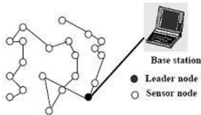
Figure 3. PEGASIS [7]
