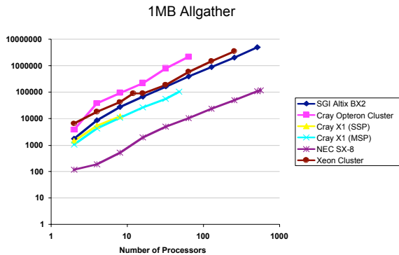
Figure 10: Execution time of Allgather benchmark on varying number of processors, using a message size of 1MB, in μs/call (i.e., the smaller the better).
