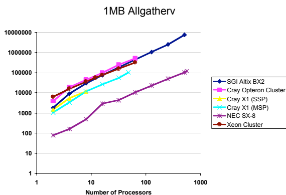
Figure 11: Execution time of Allgather benchmark on varying number of processors, using a message size of 1MB, in μs/call (i.e., the smaller the better).
