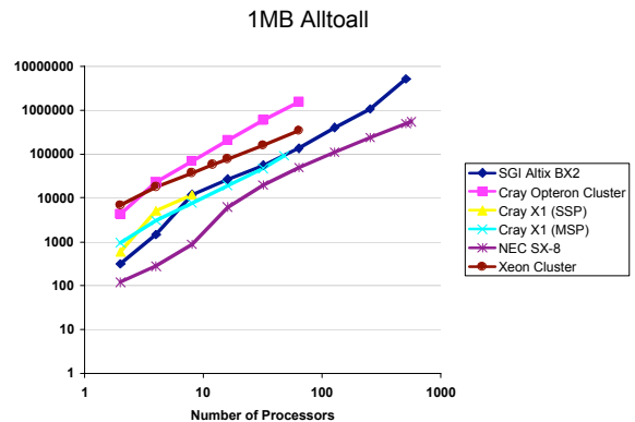
Figure 12: Execution time of AlltoAll benchmark on varying number of processors, using a message size of 1MB, in μs/call (i.e., the smaller the better).
