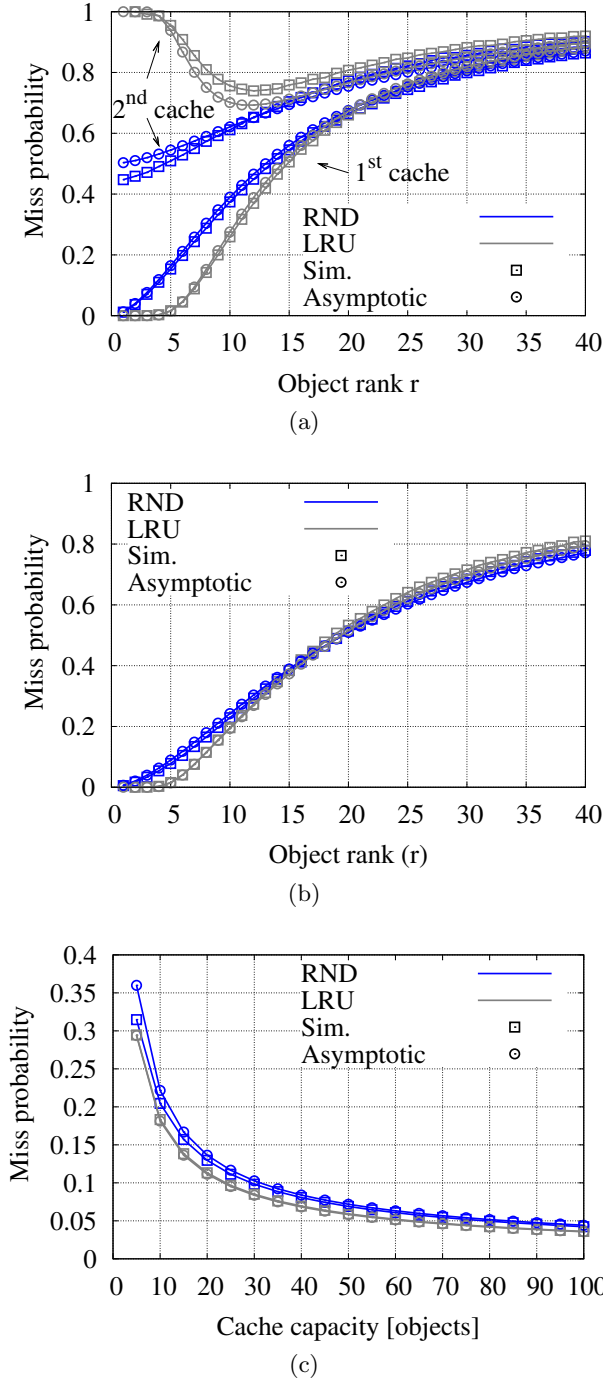
Figure 3: Tandem cache results: (a) asymptotics of M_r^*(1) , M_r^*(2) (b) and of M_r(2) for RND and LRU policies compared to simulation with C_1 = C_2 = 25 , \alpha = 1.7 (c) Asymptotic for M(2) = M(C_1, C_2) with C_1 = C_2 \leq 100 , \alpha = 1.7 .
