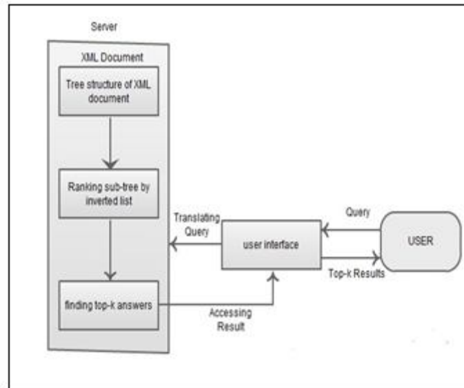
Fig 3.1 Architecture of top-k results
