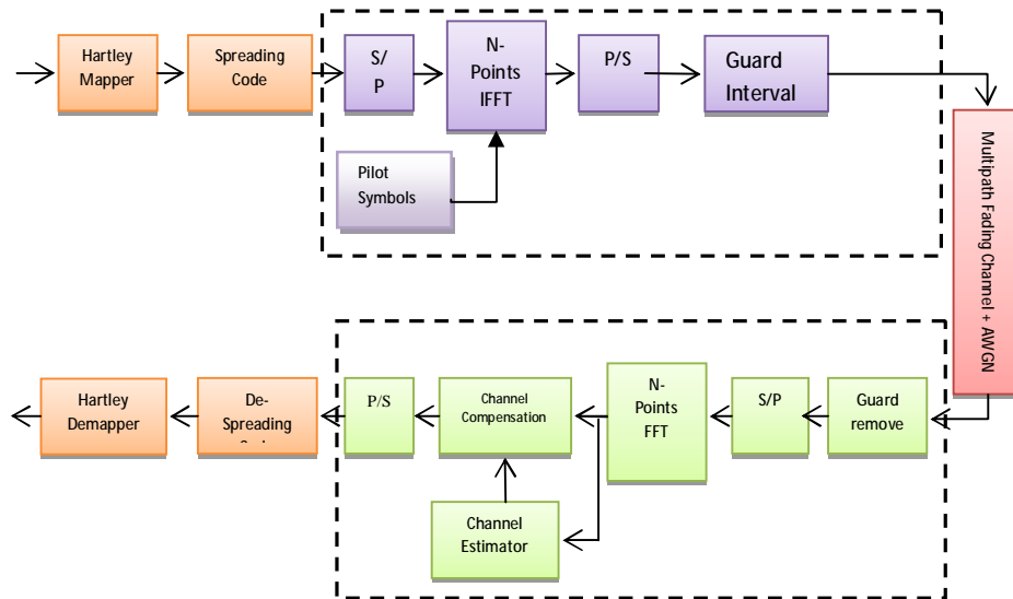
Figure (2) A proposed Hartley based MC-CDMA transceiver block diagram.
