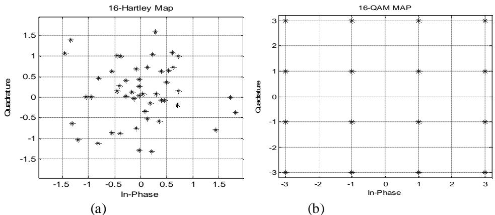
Figure (4) Constellation diagrams of the 16-Hartley, and 16-QAM mappers: (a) 16-Hartley mapper (b) 16-QAM mapper.
