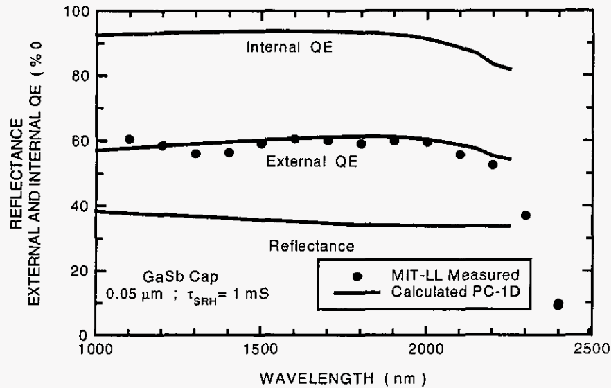
FIGURE 5. Simulated and Measured QE of GaInAsSb (0.55 eV) TPV Cell.
