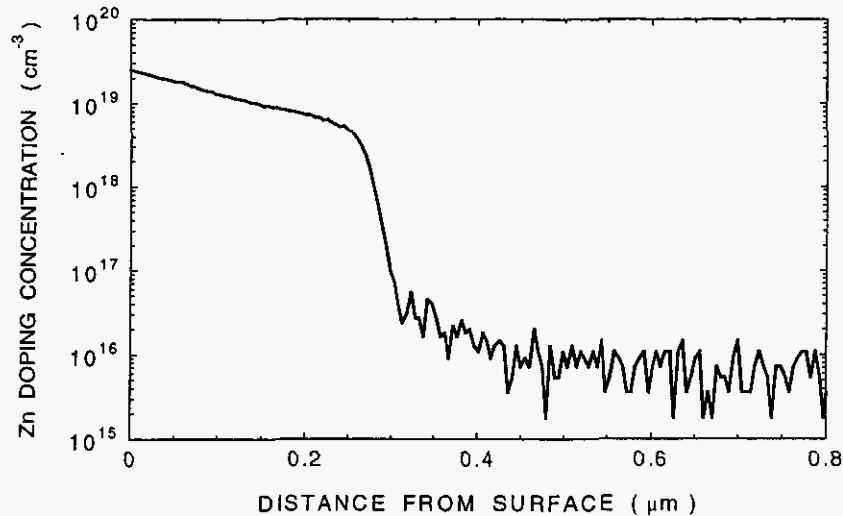
FIGURE 2. SIMS Emitter Doping Profile of Zn Bulk Diffused Cells
