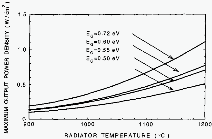
FIGURE 4. Maximum Output Power Density vs. Radiator Temperature
