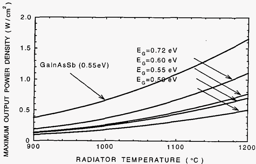
FIGURE 7. Maximum Output Power Density vs. Radiator Temperature
