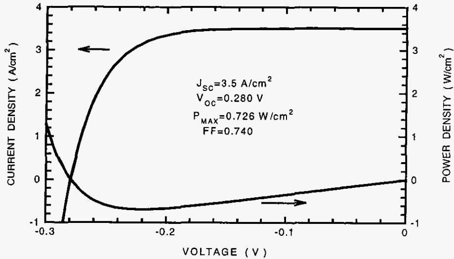
FIGURE 6. Simulated Light I-V Characteristics of GaInAsSb TPV Cell.
