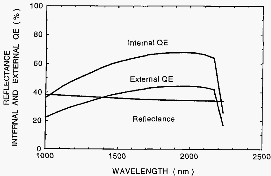
FIGURE 3. Simulation of Internal and External QE of GaInSb (0.55 eV) Cell.
