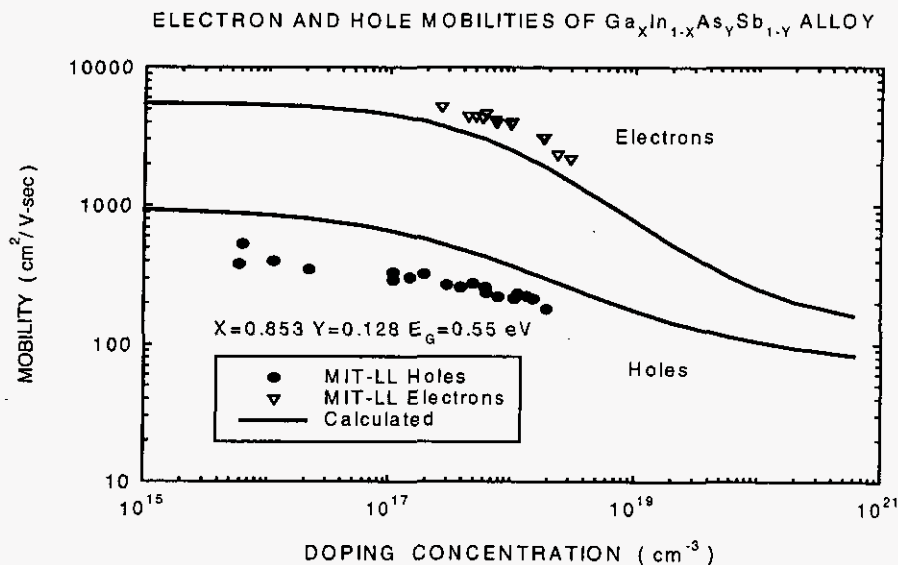
FIGURE 1. Electron and Hole Mobility of GaInAsSb Alloy.
