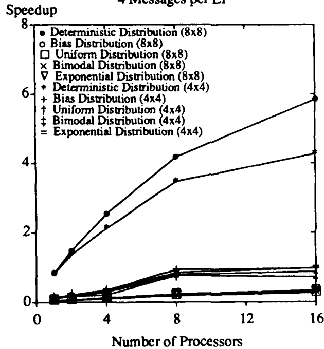
Figure 4. Speedup using deadlock detection and recovery.
