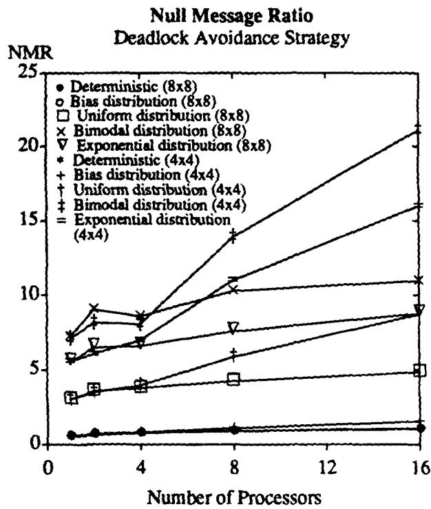
Figure 5. Overhead in deadlock avoidance simulator.
