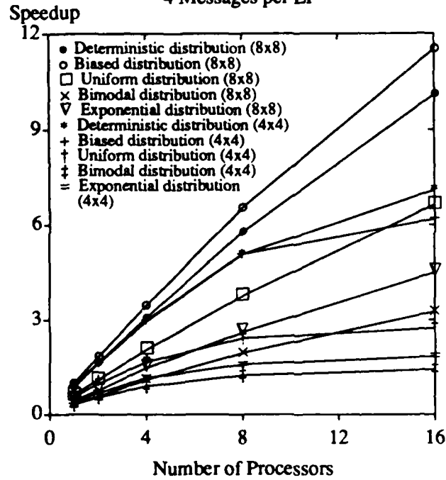
Figure 3. Speedup using deadlock avoidance.
