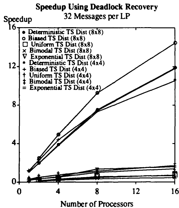
Figure 20. Speedup with high message population — deadlock recovery.
