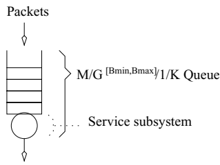
Fig. 1 The queueing model
