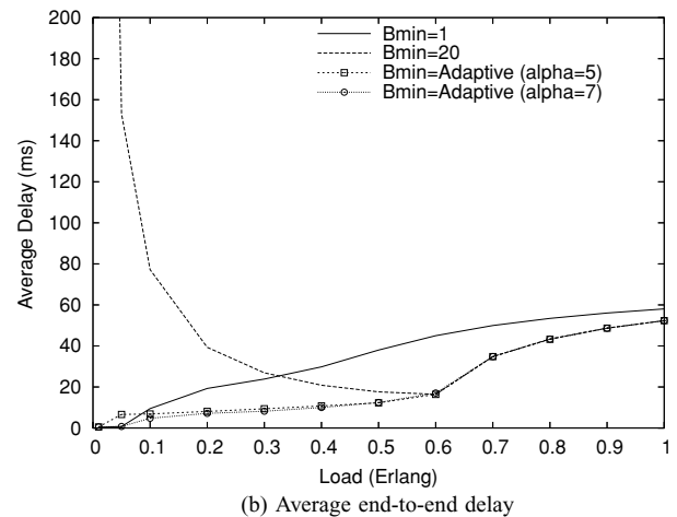
Fig. 9 Performance of the adaptive burst assembly policy
