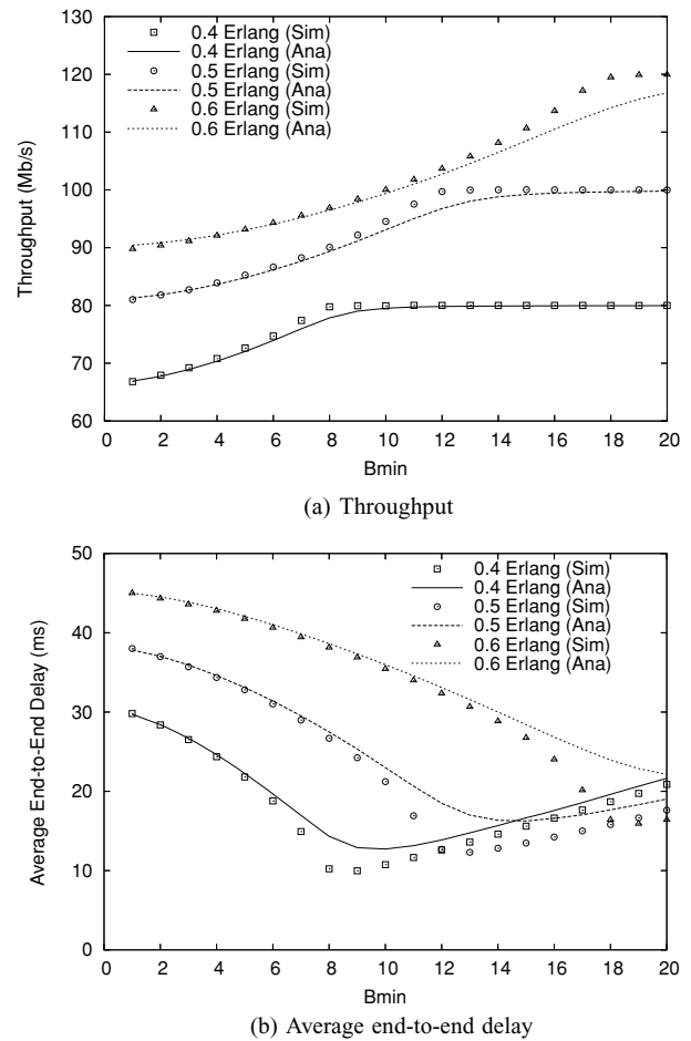
Fig. 7 Performance versus B_{\text{min}} ( N = 20 , T_{\text{sync}} = 100 \mu\text{s} , R = 200 \text{ Mb/s} , B_{\text{max}} = 20 )
