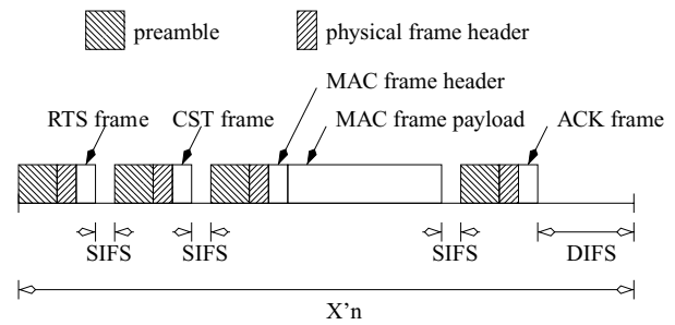
Fig. 4 Timing in a slot of successful transmission with the RTS/CTS access scheme
