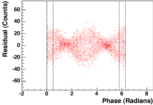
Fig. 31. The “bow-tie” effect: Variation of the residual versus the phase of the test tone. The size of the bow-tie effect was determined from the standard deviation of the fit residuals in the bands indicated from 0 \rightarrow 0.5 and 2\pi - 0.5 \rightarrow 2\pi .
