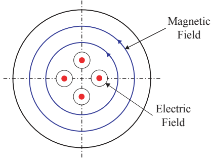
Fig. 1. The fields of the TM_{010} or monopole mode. The amplitude of the monopole mode is proportional to the bunch charge.
