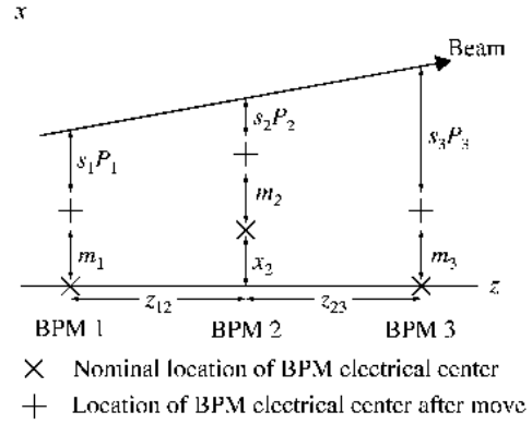
Fig. 12. The nominal positions of the electrical centers of BPMs 1 and 3 define the coordinate system, and BPM 2 is allowed to have a relative offset: These are denoted above with a \times . Each BPMs is then moved in turn away from its nominal position by a known amount m_n . The new position for the electrical center of the BPM is denoted by a + . The quantity z_{mn} is the distance between BPMs along the beamline.
