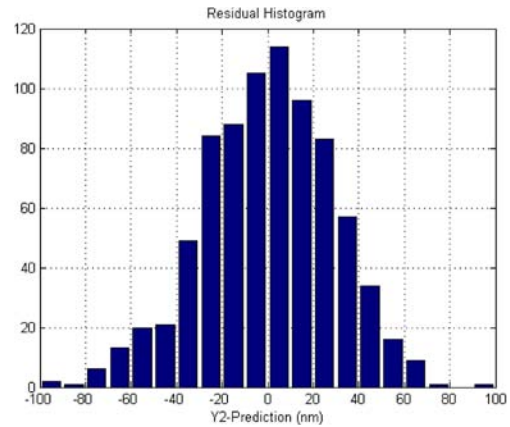
Figure 4: The residuals for 800 ATF extractions from a period spanning roughly 9 minutes on 27 May 2005. The standard deviation of the distribution was 29.4 nm and yielded a resolution of 24.0 nm.
