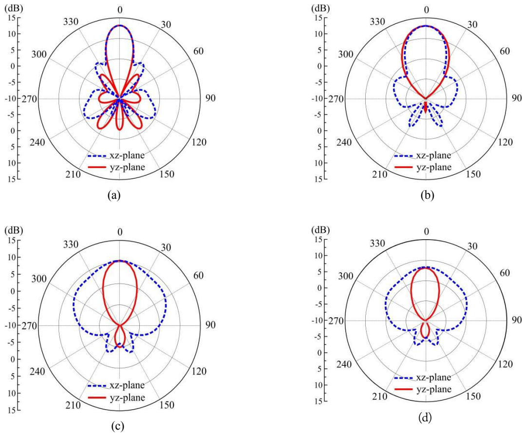
Fig. 4. Radiation patterns of the antennas: (a) H=160 \mu\text{m} at 0.316 \text{ THz} , (b) H=80 \mu\text{m} at 0.332 \text{ THz} , (c) H=40 \mu\text{m} at 0.37 \text{ THz} , and (d) H=20 \mu\text{m} at 0.38 \text{ THz} .
