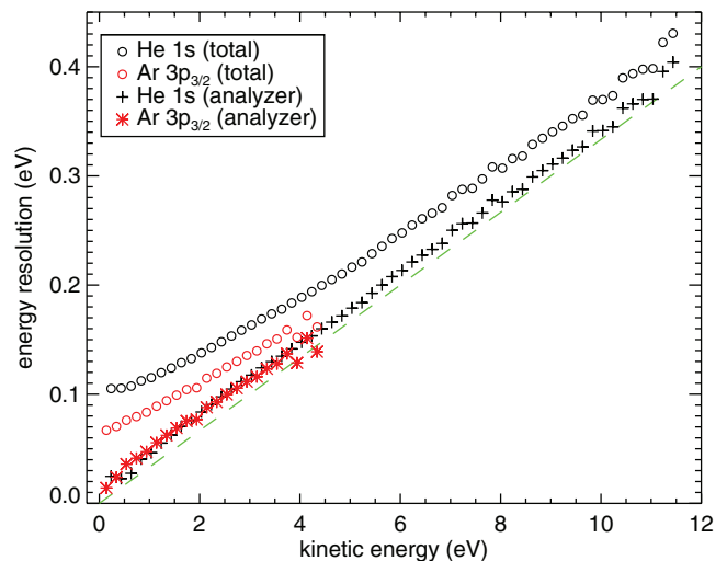
FIG. 5. Energy resolution (FWHM) of the spectrometer as a function of kinetic energy. Measurements of the atomic He 1s and Ar 3p_{3/2} photoelectron lines were analysed. Open circles show the total apparatus broadening, including spectrometer and monochromator contributions. The “pluses” and “asterisks” show the values after subtraction of an approximate monochromator broadening, see text for details. The dashed line shows the expected broadening for a spectrometer with a resolving power of E_{\text{kin}}/\Delta E_{\text{kin}} = 30 . An acceleration voltage of +1.1 V was applied to the drift tube and the entrance aperture of the spectrometer.
