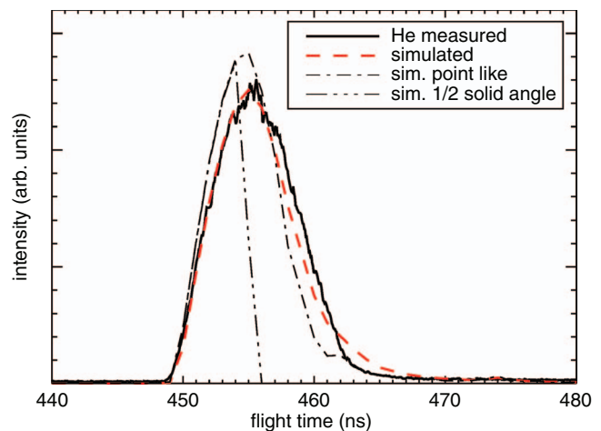
FIG. 2. Comparison of the measured time-of-flight spectrum of He 1s photoelectrons with charged particle trajectory calculations. A kinetic energy of 5 eV and an acceleration voltage of 1.1 V were chosen. The thick solid black line and the dashed lines are the measured and simulated spectra, respectively. The simulation given by the (simple) dashed line includes the effect of the finite size of the interaction region, with 3 mm extension along a line perpendicular to the spectrometer central axis, and 0.2 mm diameter in the remaining two dimensions, which is an estimate for the spatial overlap of light beam and gas jet. The other two traces were calculated under the assumption of a point-like interaction region (dash-dotted line), and under the additional restriction of admitting electron emission only into the half sphere on the drift tube side (dash-dot-dot-dotted line). The simulated traces were normalized to the same total area as the measurement (half the total area for the last trace). See text for details.
