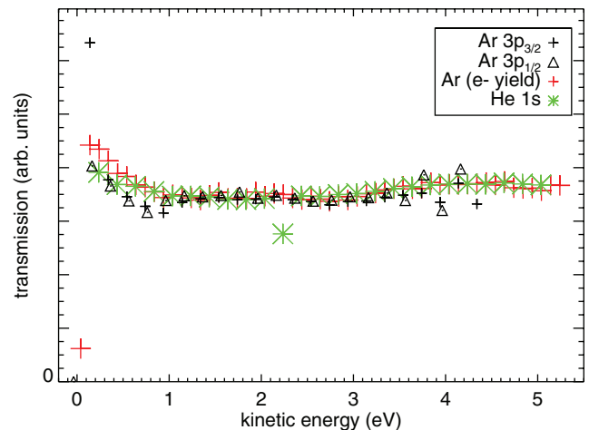
FIG. 7. Intensity of the Ar 3p_{3/2} and 3p_{1/2} photolines normalized to the ionization cross section, ring current, and the flux curve of the beamline. Resulting values reflect the kinetic energy dependence of the spectrometer transmission function, on an arbitrary scale. The lowest Ar 3p_{3/2} data point ( E_{kin} = 0.12 eV) is supposedly influenced by autoionization of Ar 3p_{1/2}^{-1}nl Rydberg states. For comparison, values from a total electron yield measurement on Ar and from measuring the He 1s photoline are shown. The latter two data sets were scaled to the average value of the Ar 3p_{3/2} data. An acceleration voltage of +1.1 V was applied to the drift tube and the entrance aperture of the spectrometer.
