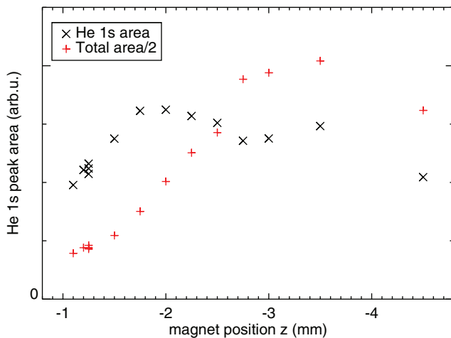
FIG. 4. Peak areas of He 1s spectra (crosses) recorded at a photon energy of 28 eV as a function of the distance between the permanent magnet and the interaction region. The total number of counts in each spectrum is also shown (plus signs), and has been divided by a factor of two for easier comparison.
