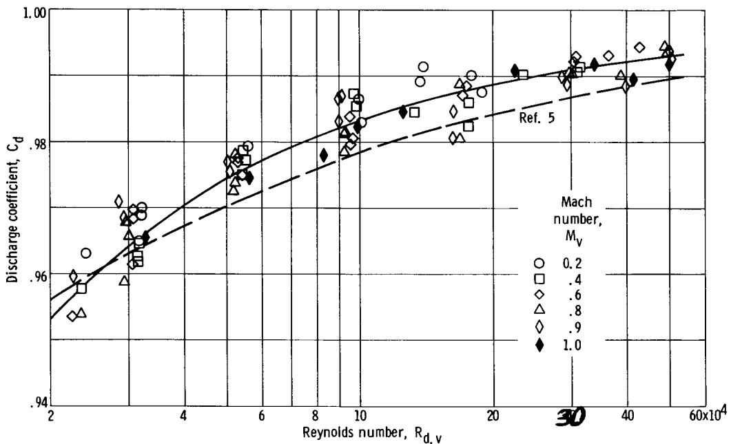
Figure 7. - Discharge coefficient as function of nozzle Reynolds number. Step size, 0; inside diameter of pipe, 2.072 inches (5.263 cm); venturi-throat diameter, 0.5025 inch (1.276 cm); ratio of throat diameter to pipe diameter, 0.242.
