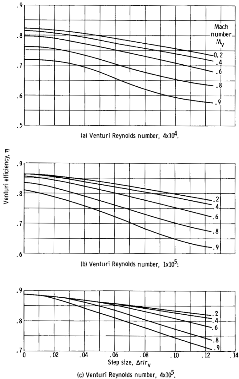
Figure 5. - Venturi efficiency as function of step size.
