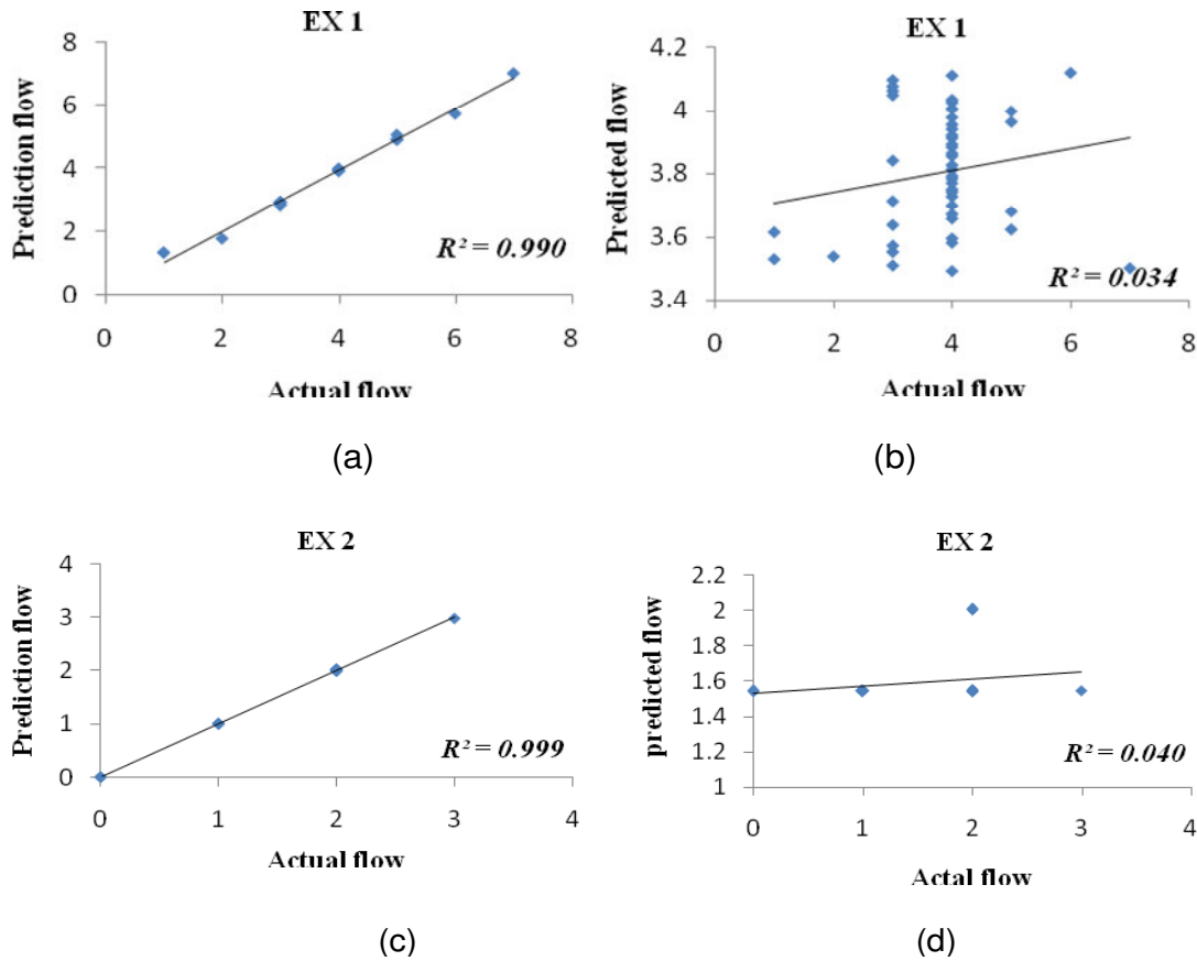
Figure 3. The performance ANN and MLR for two phases during the training process: (a) ANN-EX1; (b) MLR-EX1; (c) ANN-EX2; (d) MLR-EX2.
