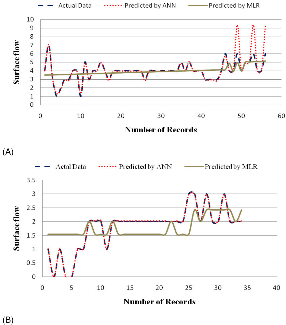
Figure 5. Comparison of ANN, MLR models and actual flow for phase (A) EX1 and (B) EX2.
