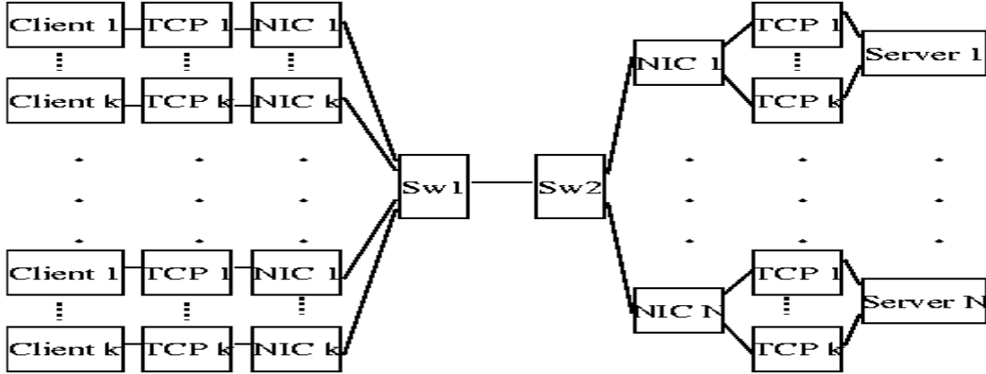
Figure 1: K-N Client-Server configuration
