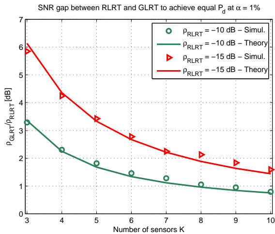
Fig. 3. SNR gap for GLRT to achieve the same P_d as RLRT, as a function of K for different levels of signal strength ( \rho_{\text{RLRT}} ). Simulation results vs. analytical approximation (30). Fixed false alarm rate \alpha = 1\% , N = 100 .
