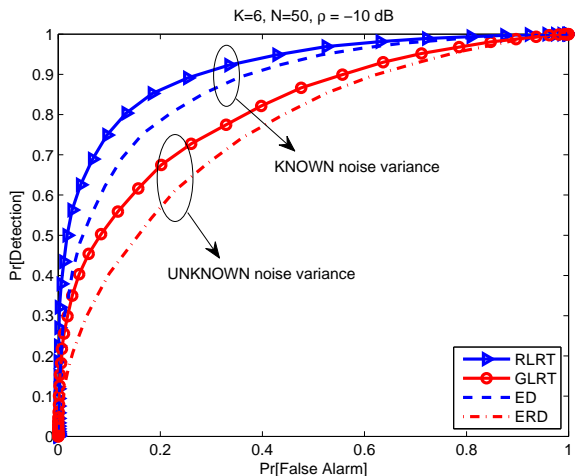
Fig. 1. Simulated receiver operating characteristics (ROC) curves for detection methods with known and unknown noise variance.
