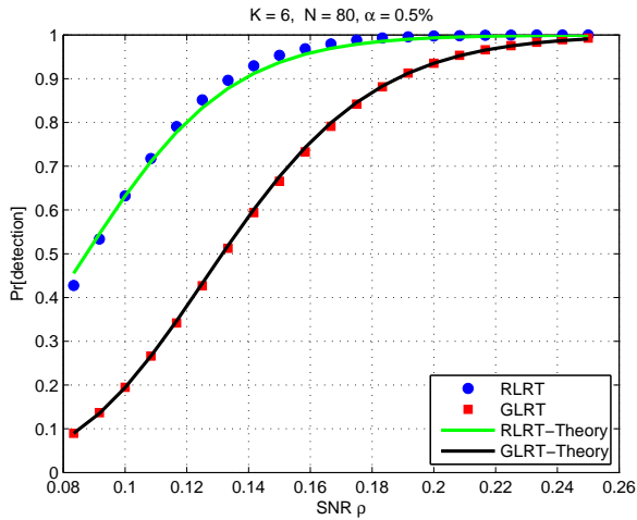
Fig. 2. Comparison of detection performance curves of RLRT and GLRT methods, from simulation and analytical expressions (20) and (26).
