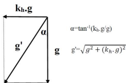
Figure 5. Acceleration resultants of the virtual gravity
