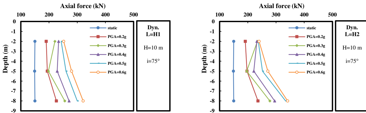
Figure 10. Dynamic axial forces of the anchors along the height of the model H10-i75
