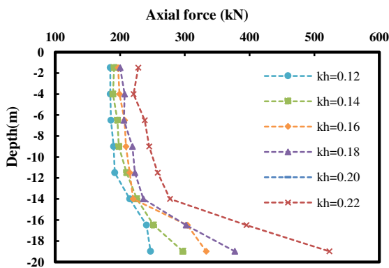
Figure 19. Pseudo-static axial forces of the anchors along the height of the model H20-i75
