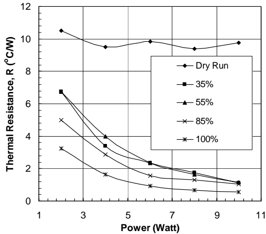
Fig. 17: Variations of thermal resistances with varying heat loads for Acetone
