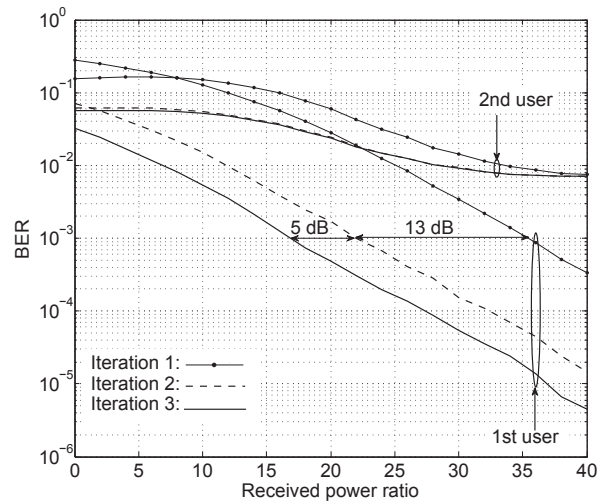
(b) 256-QAM. 2 nd user's average received SNR=35dB.
