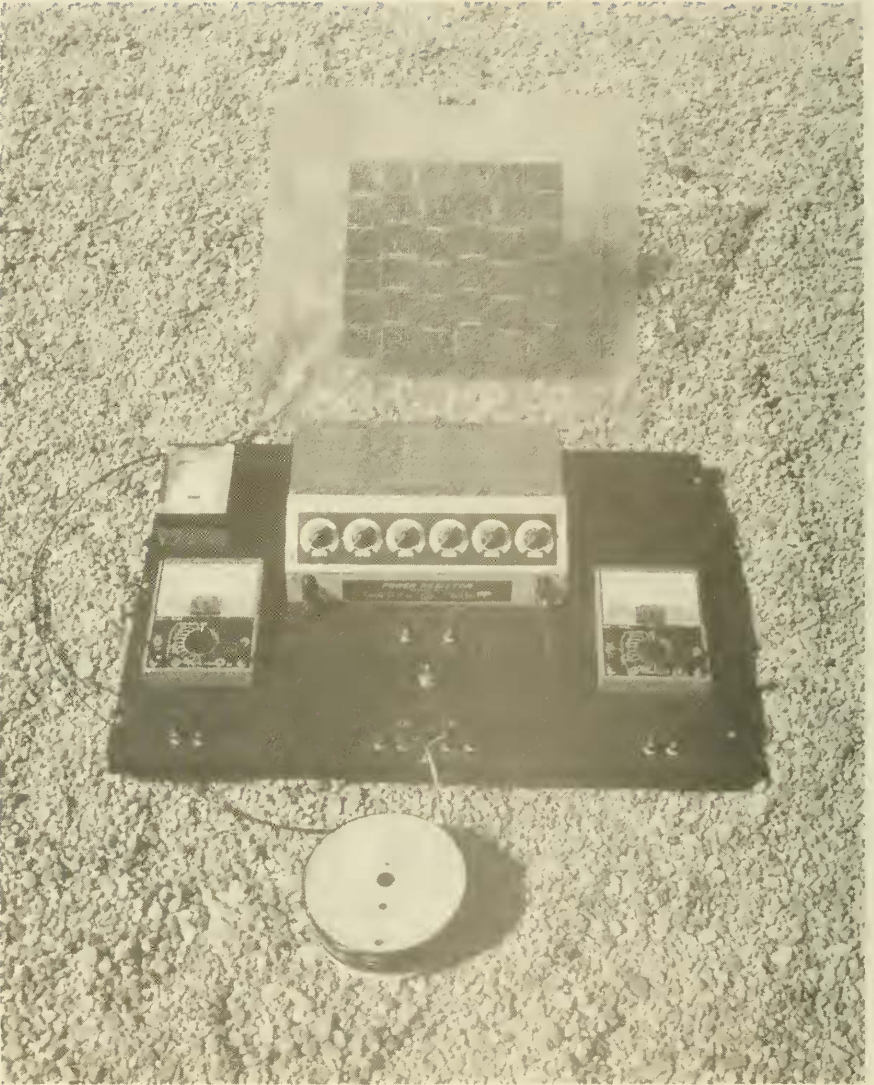
Figure 10. Equipment utilized for measurement of electrical power output by submerged solar cells. The variable resistance box allowed varying the magnitude of the electrical load across the leads from solar cells.
