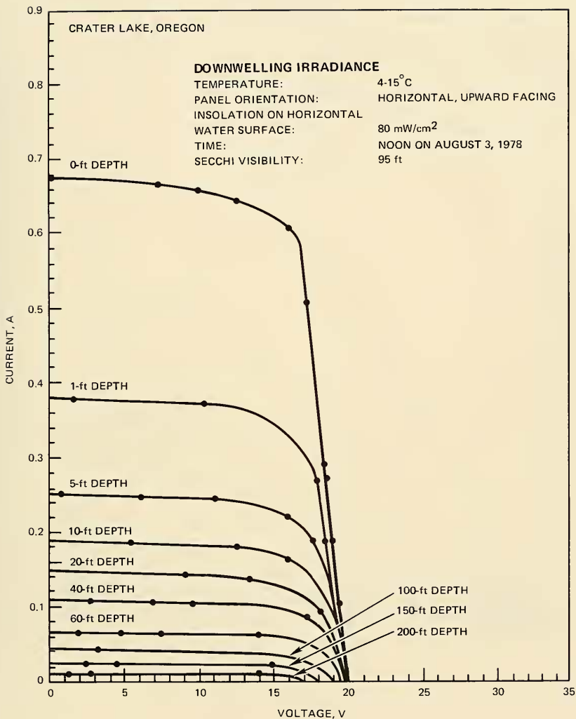
Figure 15. Voltage and current generated by the horizontal, upward-facing solar cell panel at different depths in Crater Lake, Oregon. The average Secchi disc visibility was 95 ft.
