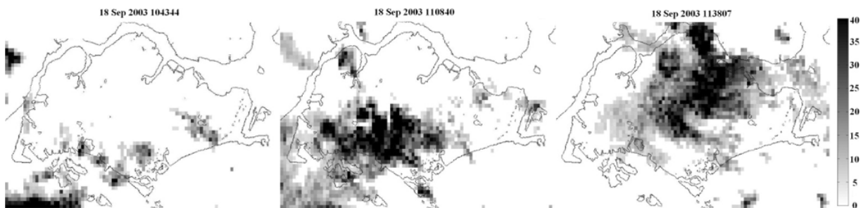
Fig. 10. CAPPI images at 500 m a.s.l. on 18 Sep. 2003(10:43–11:38)—Sumatra squall.
