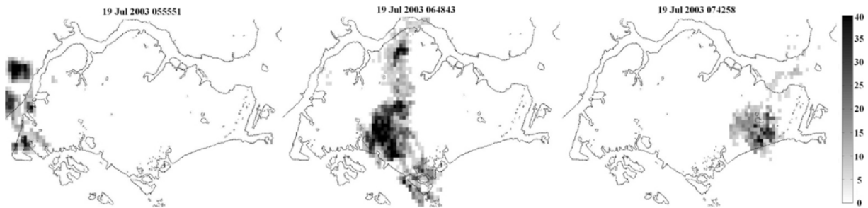
Fig. 9. CAPPI images at 500 m a.s.l. on 19 Jul. 2003 (05:55–07:42)—Rain cell elongated in the direction of the wind.
