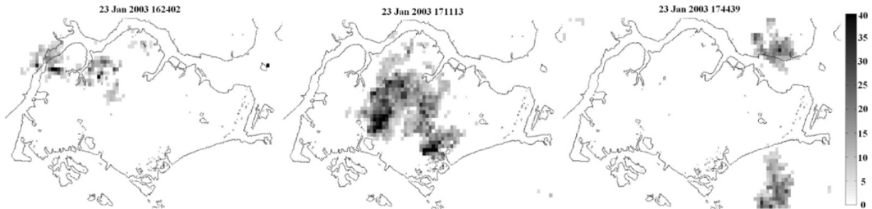
Fig. 8. CAPPI images at 500 m a.s.l. on 23 Jan. 2003 (16:24–17:44)—Rain cell moves in the direction of the wind.
