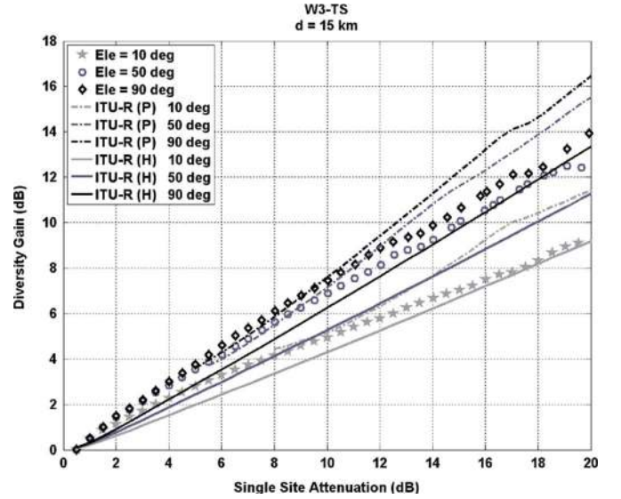
Fig. 5. Effect of Elevation Angle ( F = 18.9 GHz; Distance = 15 km; pol = V ).
