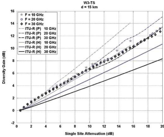
Fig. 4. Effect of Frequency (Distance = 15 km; \theta = 44.5^\circ ; pol = V ).
