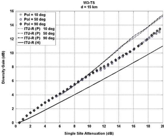
Fig. 6. Effect of Polarization ( F = 18.9 GHz; \theta = 44.5^\circ ; Distance = 15 km).
