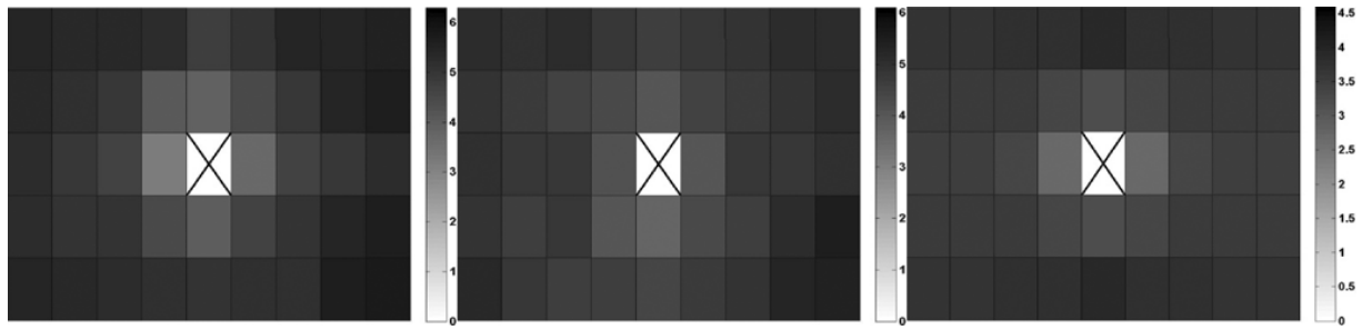
Fig. 7. Site Diversity Gain around Singapore (Left: 1 year simulated result; Middle: Paraboni-Barbaliscia model predicted result; Right: Hodge model predicted result).
