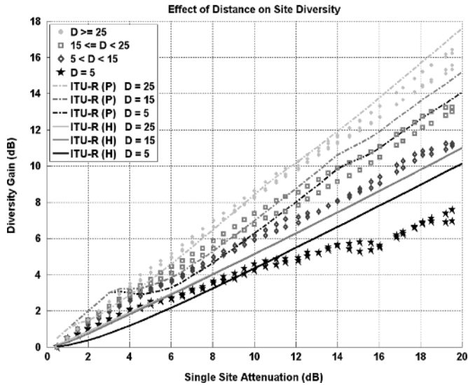
Fig. 3. Effect of Site Separation ( F = 18.9 GHz; \theta = 44.5^\circ ; p_{0.1} = V ).
