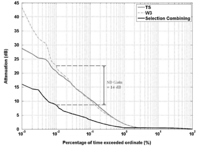
Fig. 2. CDF of Attenuation of Single Site W3 and TS and Selection Combining of Two Sites.
