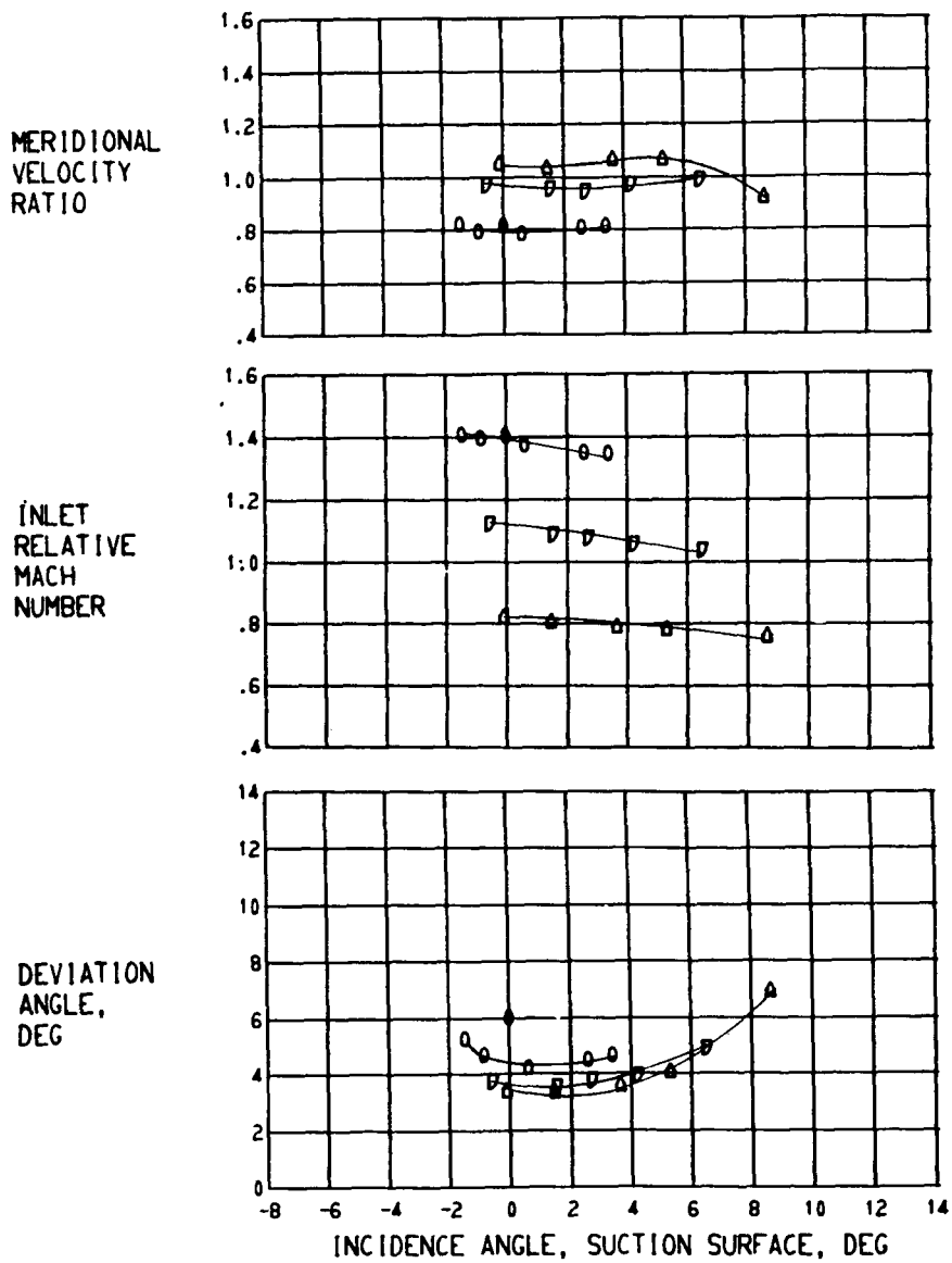
(B) CONTINUED. 10.0 PERCENT SPAN. FIGURE 10 - BLADE ELEMENT PERFORMANCE FOR ROTOR NO. 7
