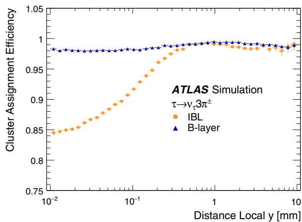
(c) \tau \rightarrow \pi^+ \pi^- \pi^\pm \nu_\tau sample
