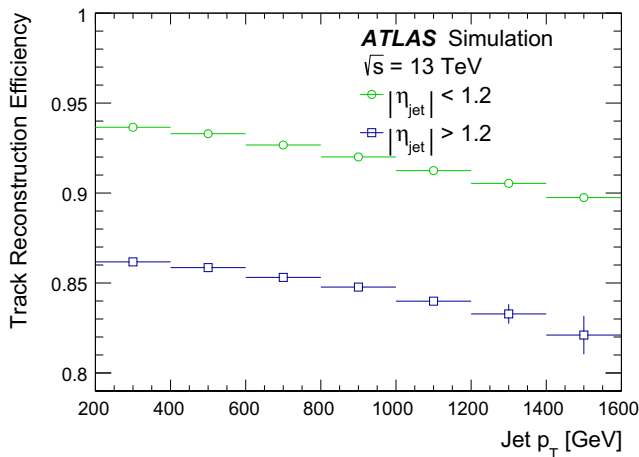
Fig. 14 The track reconstruction efficiency is compared for charged primary particles in jets with |\eta| < 1.2 ( |\eta| > 1.2 ) for the entire jet- p_T range as a function of a the jet p_T and b the production radius of the
