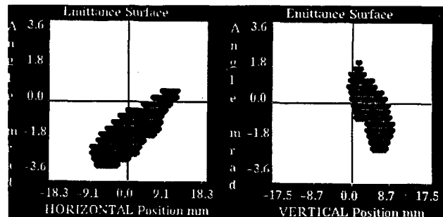
Fig. 4 Measured Linac 2 Horizontal and Vertical Emittances
