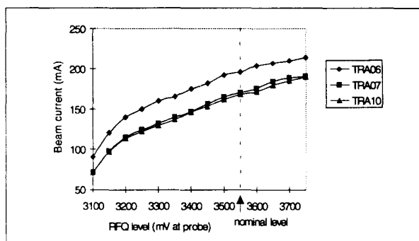
Fig. 3 Linac 2 currents as function of RFQ level
