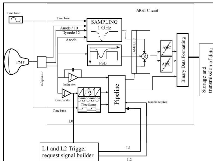
22 23 24 Figure 6. The ARS architecture. 25 26
