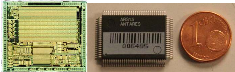
12 13 14 Figure 5. Images of the ARS chip, bare die (left) and packaged chip (right).
