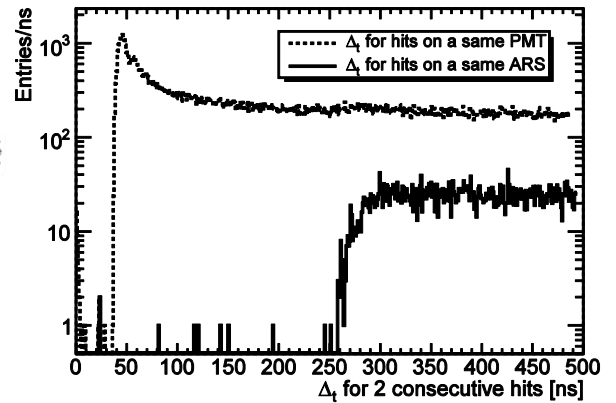
Figure 21. Time difference between two consecutive hits. Upper curve: two hits in the same PMT. Lower curve: two hits in the same ARS.
