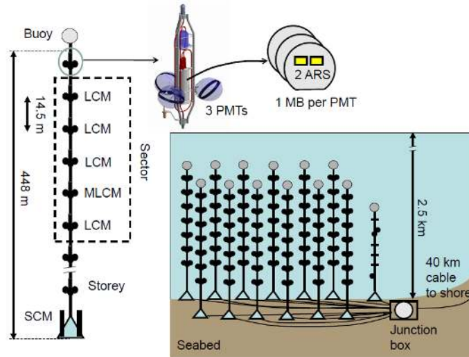
6 7 8 9 10 11 12 13 14 15 16 17 18 19 20 21 22 23 24 25 26 27 28 29 30 31 32 33 34 35 36 37 38 39 40 41 42 Figure 1. Schematic view of the ANTARES detector.
