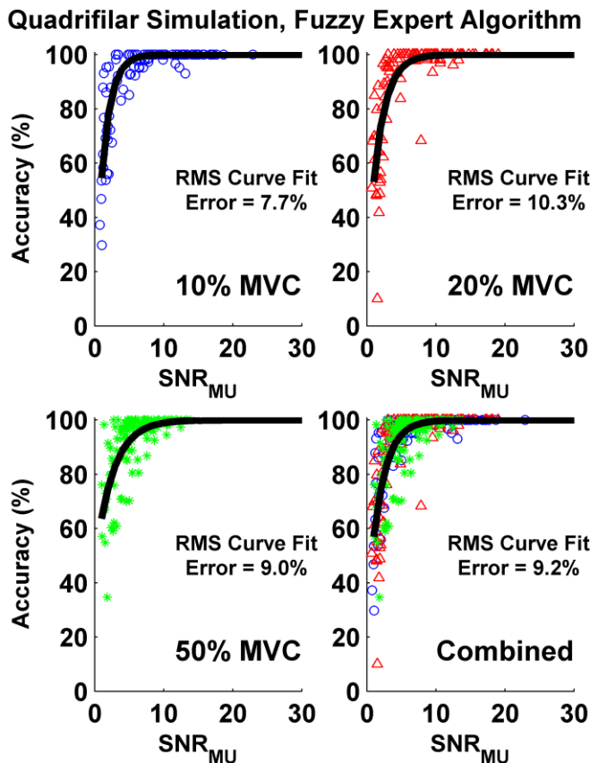
Fig. 3. Accuracy with respect to the true decomposition for the simulated quadrifilar data as a function of SNR_{MU} for the Fuzzy Expert algorithm. Each point represents one MUAPT. Results shown separately for each MVC level, and for all levels combined. Best fit exponential model shown in each plot, along with the RMS fit error.
