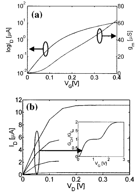
FIG. 2. I - V characteristics of the coaxially gated CNTFET. (a) Computed \log(I_D) vs V_G (on the left axis) and transconductance vs V_G (on the right axis) at V_D = 0.4 V. (b) The computed I_D vs V_D characteristic with gate bias as a parameter. ( V_G = 0.1 – 0.4 V, 0.1 V/step.) The inset shows the quantized channel conductance vs gate voltage at T = 300 K. The normalization conductance G_0 = 4e^2/h , where e is the electron charge and h the Planck constant.
