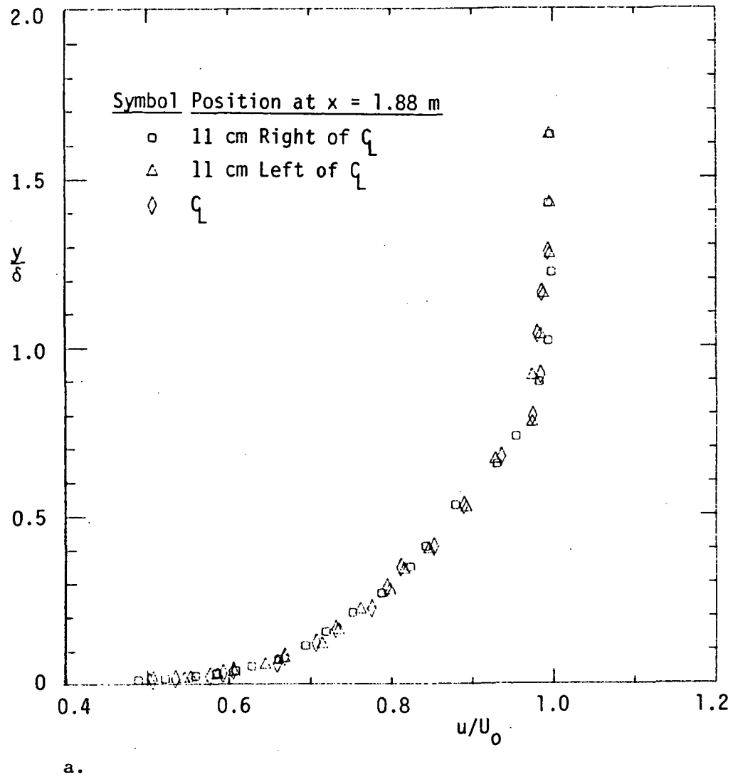
Figure 8. Experimental results for three boundary layer surveys at x = 1.88 m. (See Figure 3 for left and right designations.)
