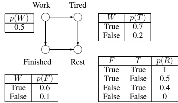
Figure 1: The work-rest Bayesian Network
