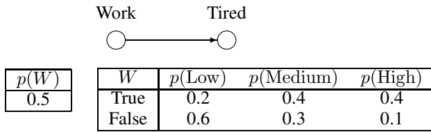
Figure 3: A Bayesian network example with a multiple valued node.
