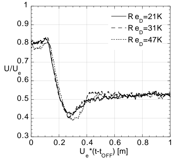
Figure 22b: Effect of Re_D on jet response to a step change in \langle c_\mu \rangle (2.4-0.0%) at x/D=1.6 , z/D=0.0 , and U/U_e=0.5 . \theta=30^\circ , L=1.85D X-diffuser. OFF.
