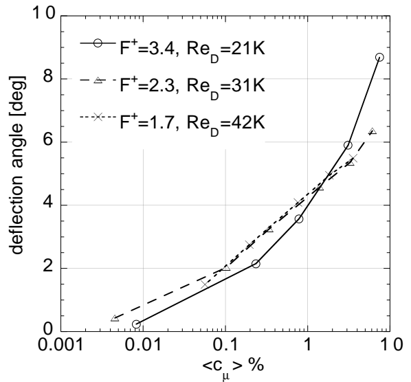
Figure 8: The effect of Re_D on jet deflection angle measured at x/D=2.5 and z/D=0.0 ( \phi = 30^\circ , L = 1.0D X-diffuser).
