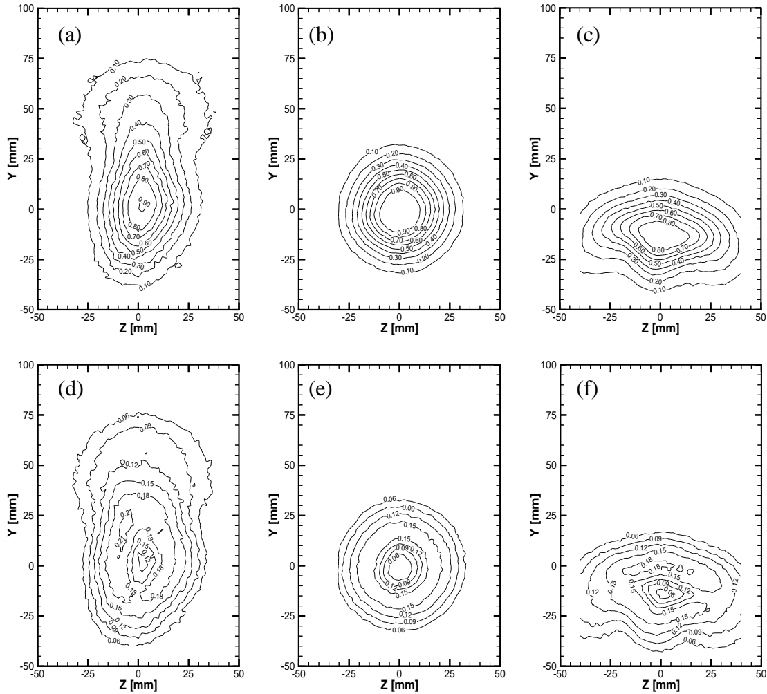
Figure 6: U/U_e and u/U_e contours at x/D=2.5 Re_D=3.1 \times 10^4 for different excitation directions (a) U/U_e , streamwise excitation, \langle c_\mu \rangle = 3.3\% , F^+ = 2.3 , L = 1.0D (b) U/U_e , baseline (c) U/U_e cross-stream excitation \langle c_\mu \rangle = 3.3\% , F^+ = 4.2 , L = 1.85D , (d) u/U_e , streamwise excitation, \langle c_\mu \rangle = 3.3\% , F^+ = 2.3 , L = 1.0D (e) u/U_e , baseline, and (d) u/U_e , cross-stream excitation, \langle c_\mu \rangle = 3.3\% , F^+ = 4.2 , L = 1.85D .
