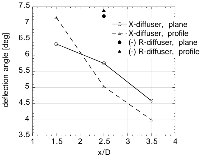
Figure 7: Jet deflection angles computed using profiles on z/D=0.0 , and cross-section planes. \langle c_\mu \rangle = 3.3\% , F^+ = 2.3 , and L = 1.0D for X-diffuser. \langle c_\mu \rangle = 3.3\% , F^+ = 4.2 and L = 1.85D for R-diffuser. Re_D = 3.1 \times 10^4 .
