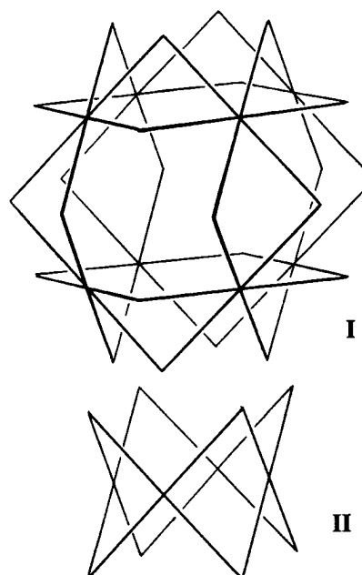
Figure 4. Diad frameworks for Im\bar{3}m-Pm\bar{3}m .
