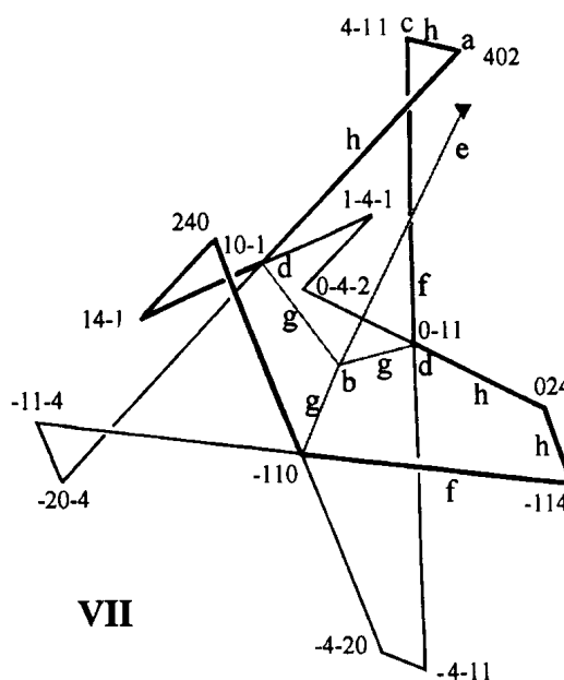
Figure 9. Diad framework for I4_132-P4_332 .
