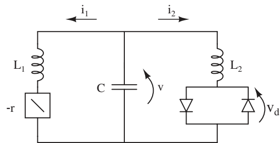
FIG. 1. The symmetric electronic circuit which displays the infinite hierarchy of nested spirals illustrated in Fig. 2. It involves negative linear and nonlinear resistive elements.
